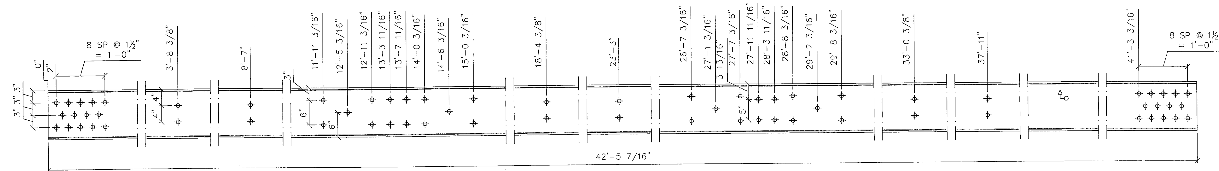
4 - BOTTOM CHORD - bc2 C12X30 (42'-5 7/16") WEATH
