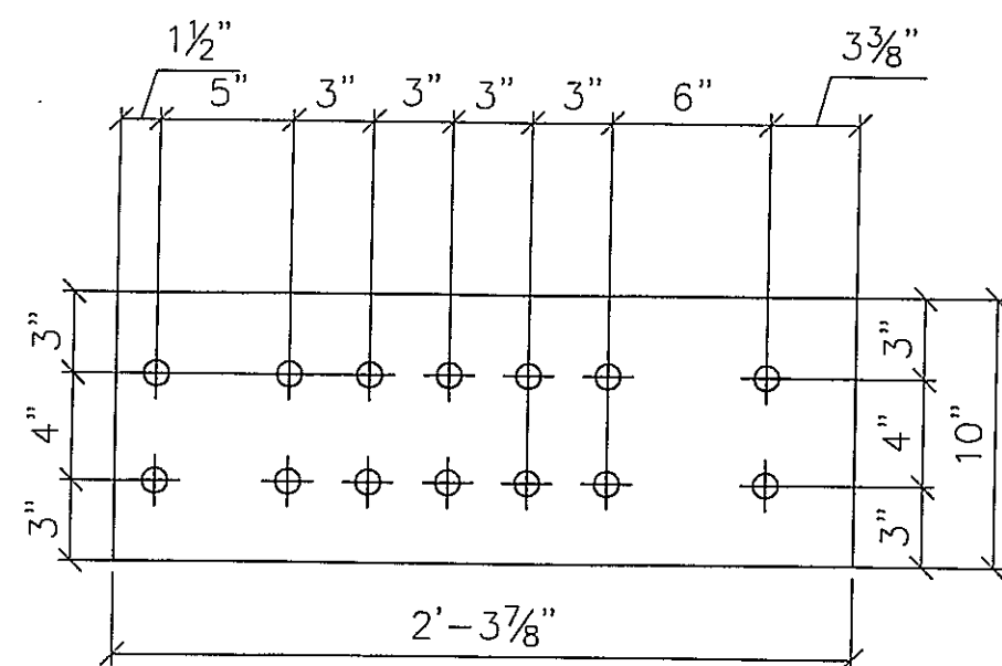
4 - FLOOR BEAM END PLATE - fbep1 Plate 3/4"x10"x2'-3 7/8" (GALV)
