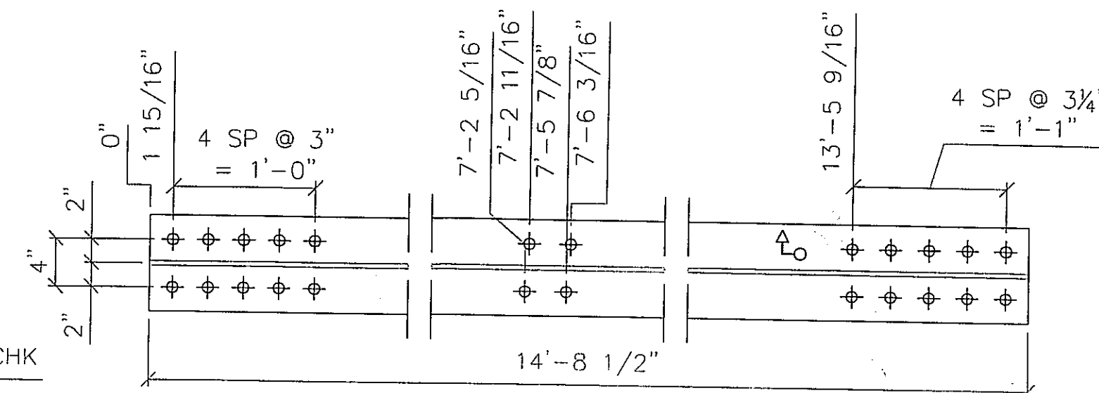
4 - TOP CHORD - tc3 W12X50 (14'-8 1/2") WEATH
