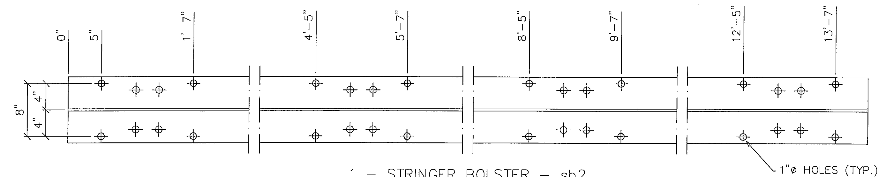
1 - STRINGER BOLSTER - sb2 W12X53 (14'-0") GALV
