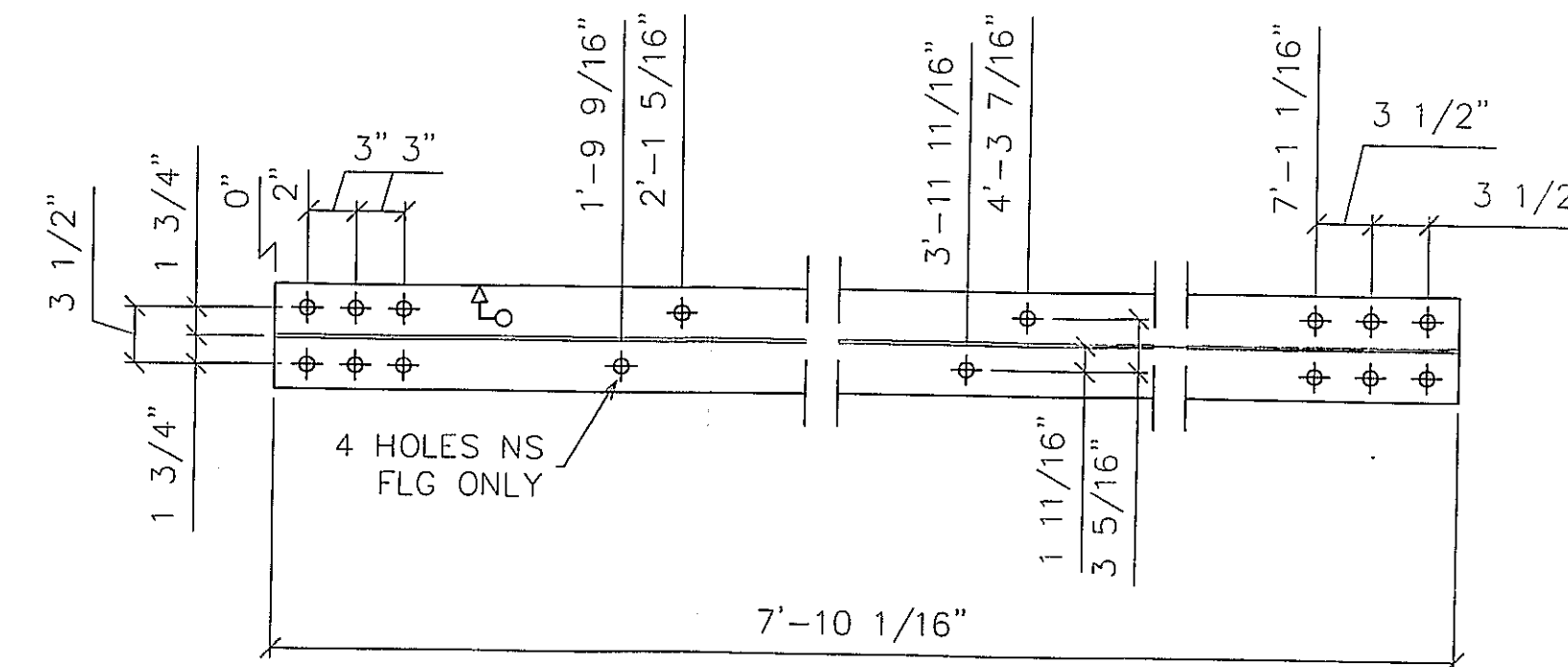
2 - DIAGONAL BRACE - d1 W12X26 (7'-10 1/16") WEATH
