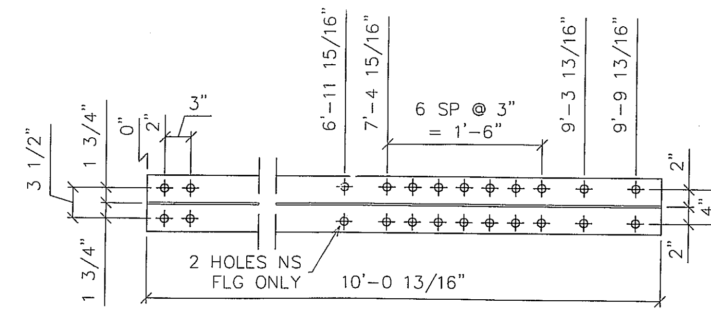
2 - VERTICAL BRACE - v3 W12X26 (10'-0 13/16") WEATH
