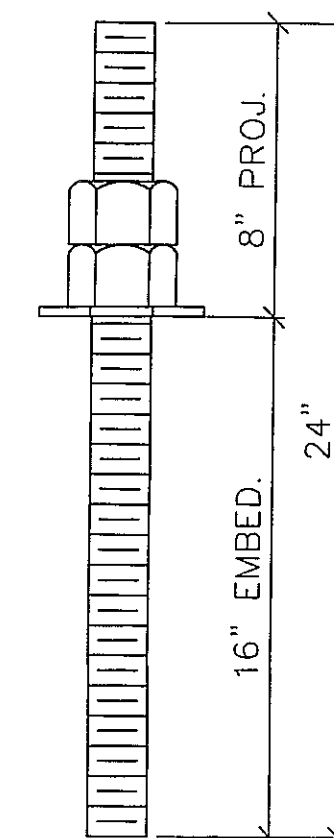
8 - TRUSS ANCHOR BOLT - AB1
