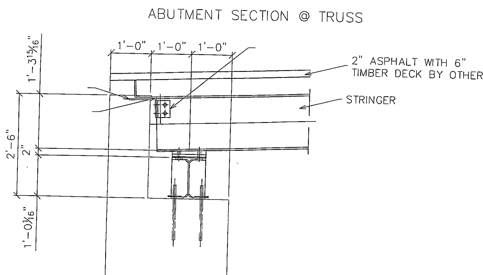
ABUTMENT SECTION @ STRINGERS
