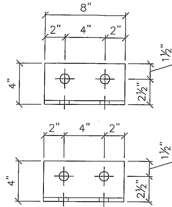
48 - BOTTOM CHORD SPACER - bcs1 L4X4X3/8 (8") WEATH
