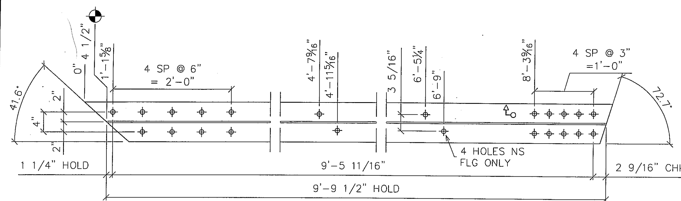
2 - TOP CHORD - tc1 W12X40 (10'-3 1/4") WEATH
