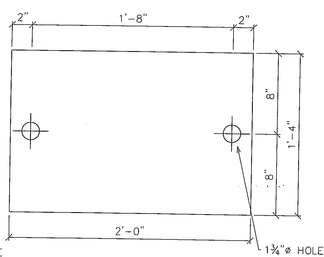
2 - BEARING PLATE - bp3 Plate 1"x1'-4" (2'-0") GALV
