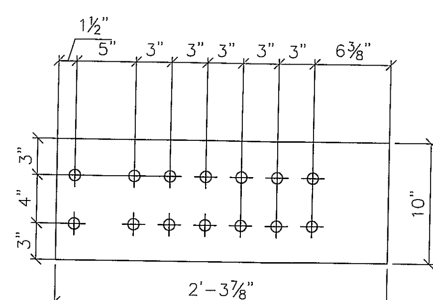
4 - FLOOR BEAM END PLATE - fbep2 Plate 3/4"x10"x2'-3 7/8" (GALV)
