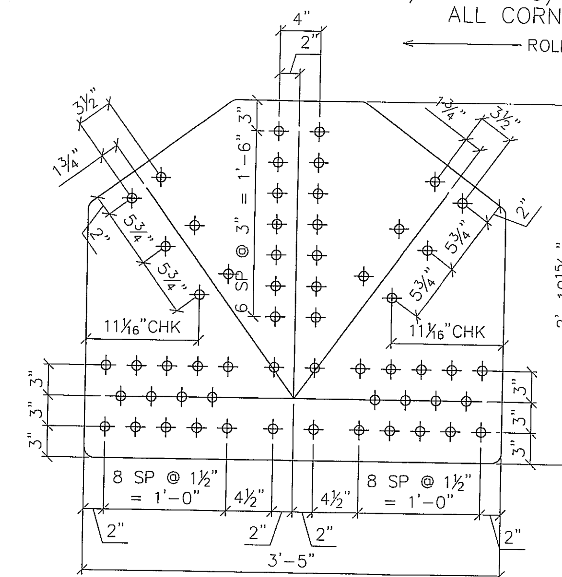
4 - LOWER GUSSET - 17 Plate 1/2"x2'-10 5/16"x3'-5 1/16" (WEATH) ALL CORNERS = 1"R UNO
