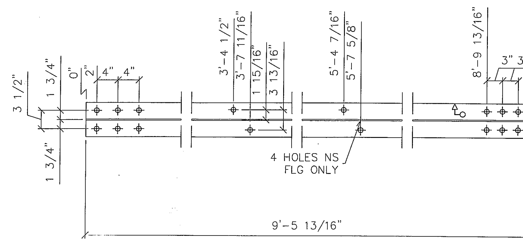
2 - DIAGONAL BRACE - d2 W12X26 (9'-5 13/16") WEATH
