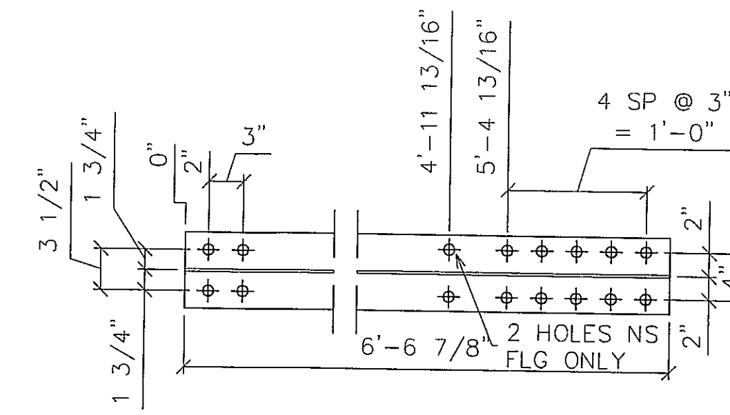
4 - VERTICAL BRACE - v1 W12X26 (6'-6 7/8") WEATH
