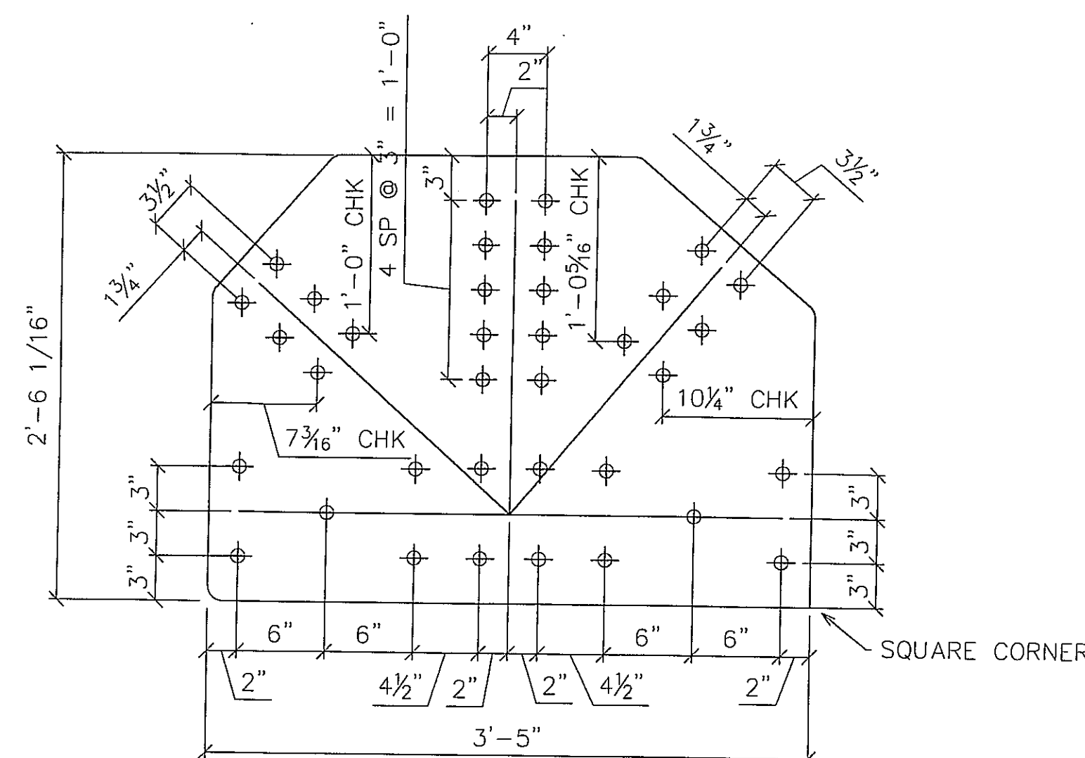
8 - LOWER GUSSET - 13111 Plate 1/2"x2'-6 1/16"x3'-5" (WEATH) ALL CORNERS = 1"R UNO
