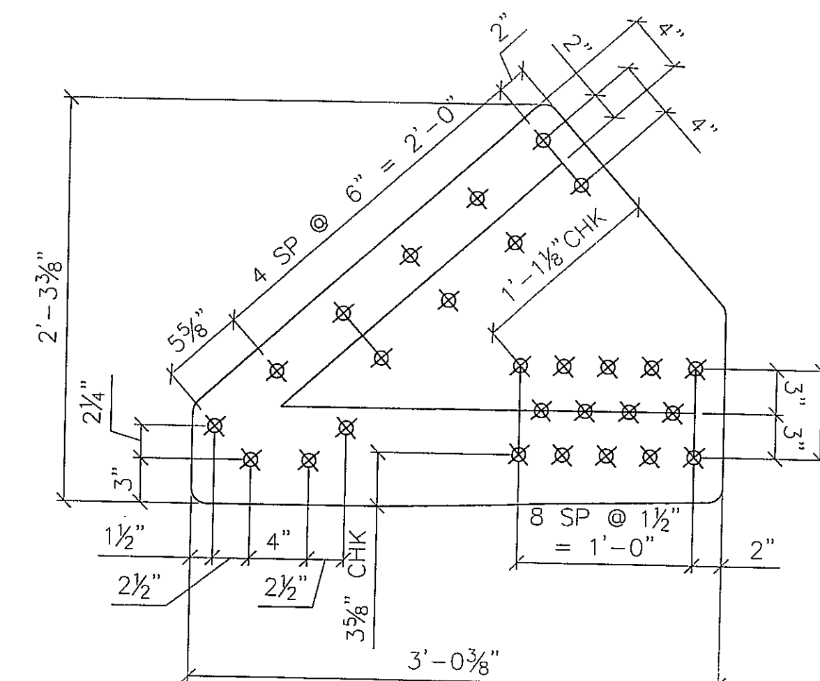
8 - LOWER GUSSET - 11113 Plate 1/2"x2'-4 3/16"x2'-11 13/16" (WEATH) ALL CORNERS = 1"R UNO
