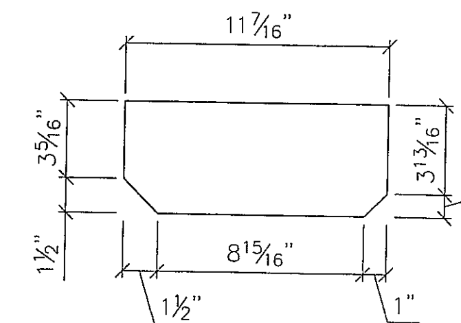
16 - BOLSTER STIFFENER - bs1 Plate 3/8"x4 13/16" (11 7/16") GALV
