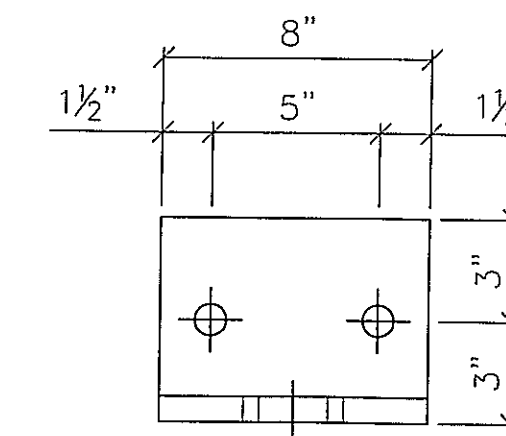
8 - BOTTOM CHORD SPACER WT - bcwt1 W10X45 (9") WEATH
