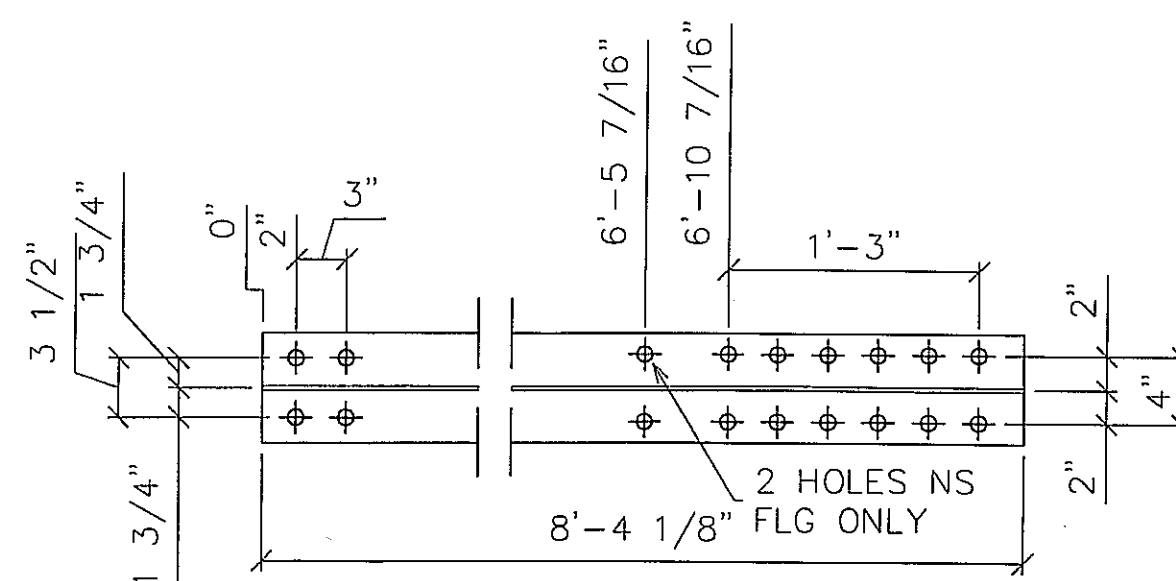
4 - VERTICAL BRACE - v2 W12X26 (8'-4 1/8") WEATH
