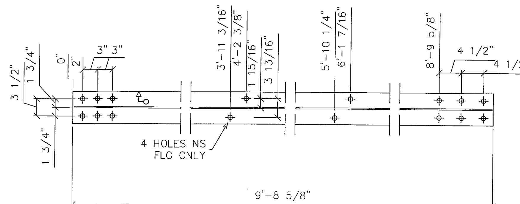
2 - DIAGONAL BRACE - d3 W12X26 (9'-8 5/8") WEATH
