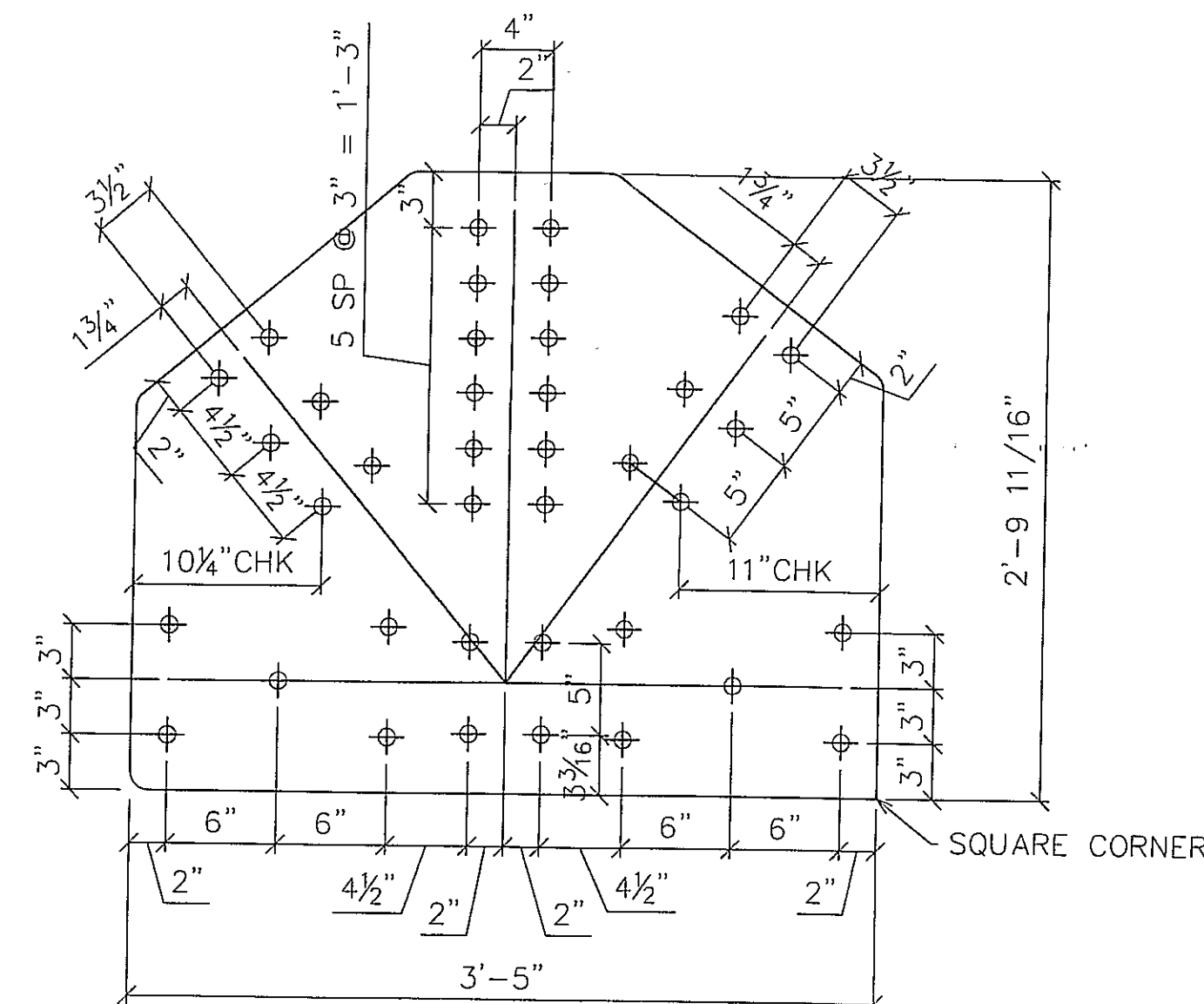
8 - LOWER GUSSET - 1519 Plate 1/2"x2'-9 11/16"x3'-5" (WEATH) ALL CORNERS = 1"R UNO
