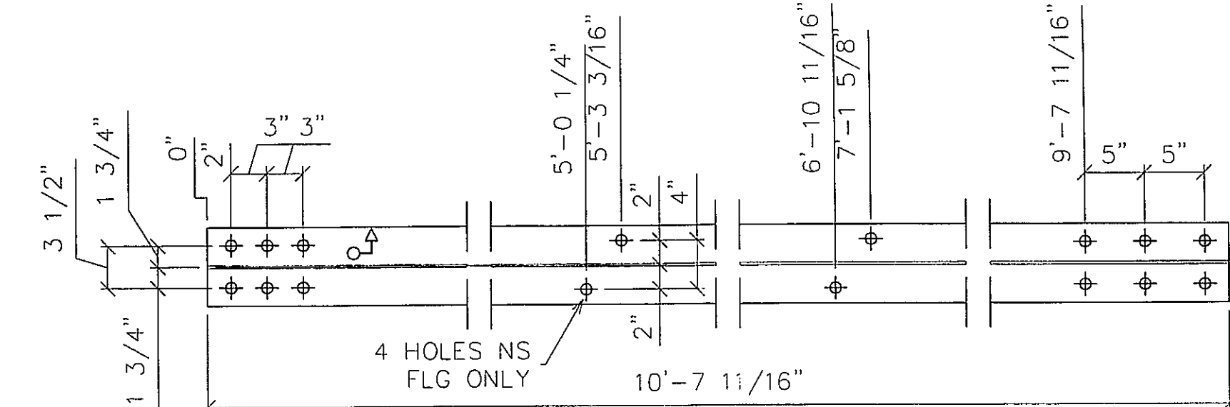
2 - DIAGONAL BRACE - d7 W12X26 (10'-7 11/16") WEATH
