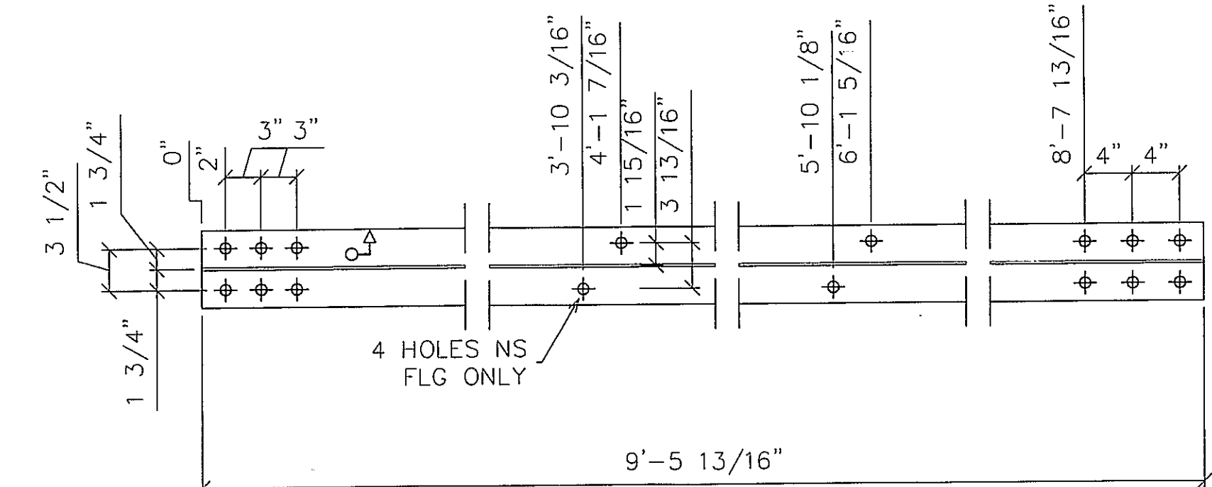
2 - DIAGONAL BRACE - d9 W12X26 (9'-5 13/16") WEATH
