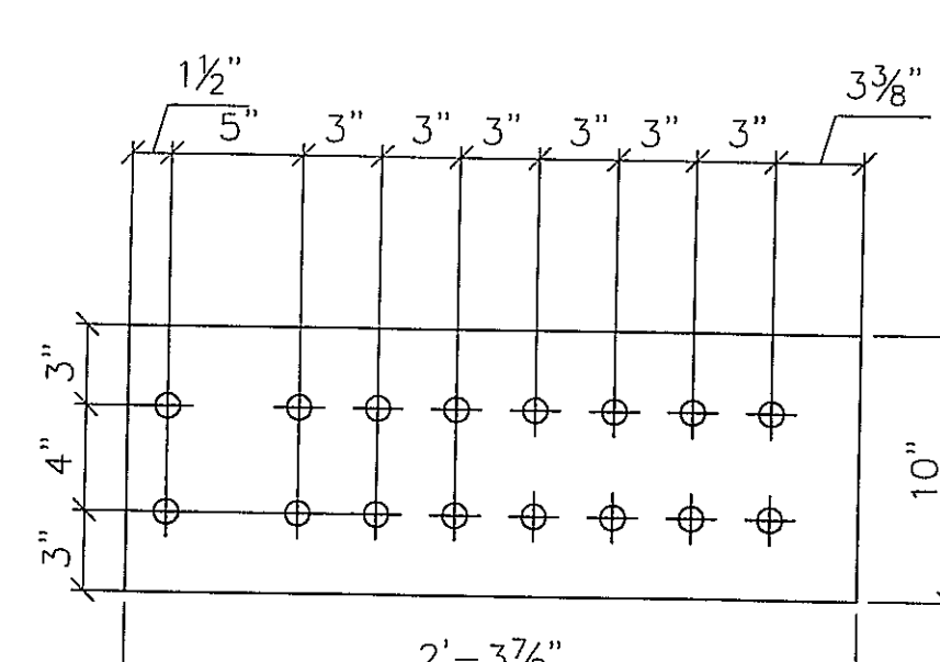
2 - FLOOR BEAM END PLATE - fbep3 Plate 3/4"x10"x2'-3 7/8" (GALV)
