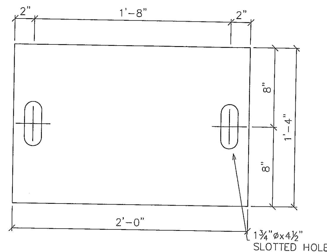
2 - BEARING PLATE - bp2 Plate 1"x1'-4" (2'-0") GALV
