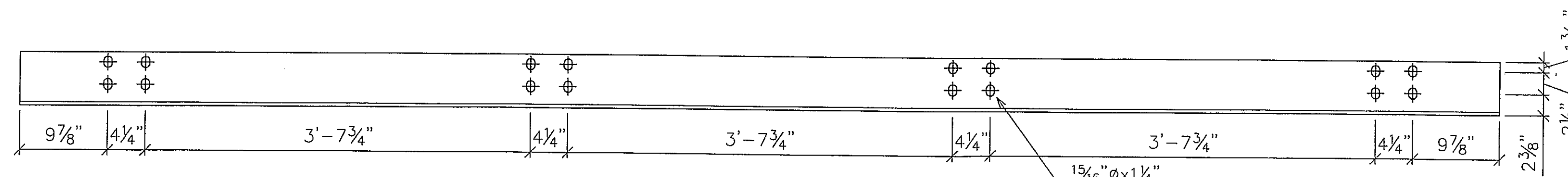
2 - SHELF ANGLE - sa1 L6X6X3/8 (14'-0") GALV
