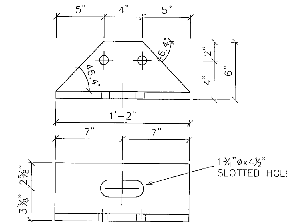
4 - TRUSS BEARING ANGLE - tba1 L6X6X3/4 (1'-2") WEATH
