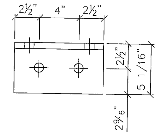
8 - BOTTOM CHORD SPACER WT - bcwt2 W10X45 (9") WEATH
