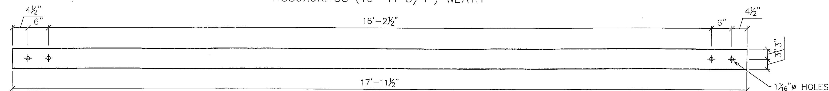
4 - GUARDRAIL - gdr2 HSS6X6X.188 (17'-11 1/2") WEATH
