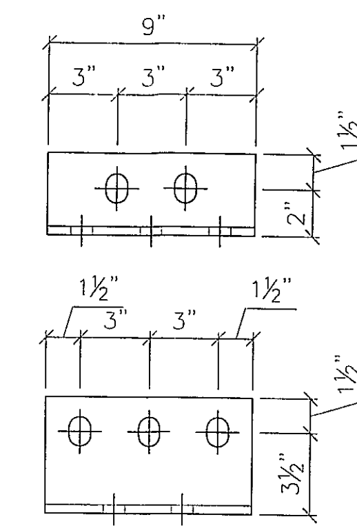
80 - STRINGER CONNECTION ANGLE - sca2 L5X3-1/2X3/8 (9") GALV
