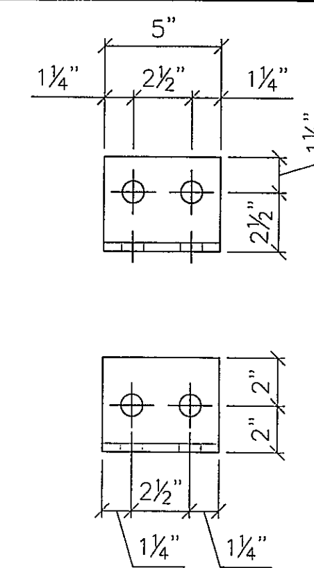
16 - STRINGER CONNECTION ANGLE - sca1 L4X4X3/8 (5") GALV
