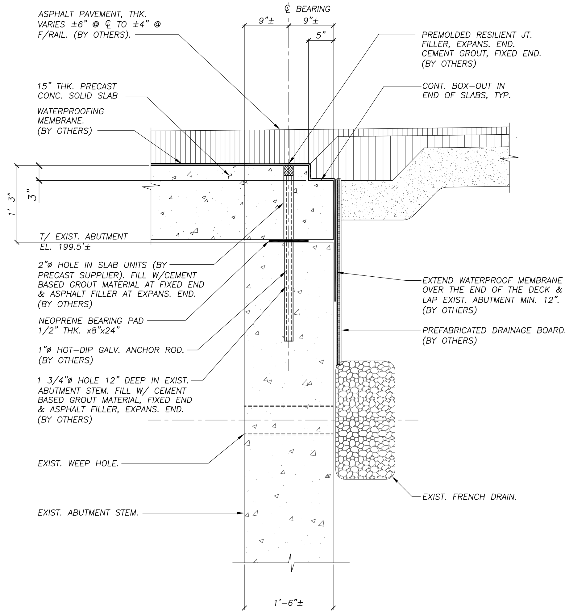
SECTION 3 1"=1'-0" NOTE: EXPANSION END SHOWN, FIXED END SIMILAR. SEE DETAIL NOTES.
