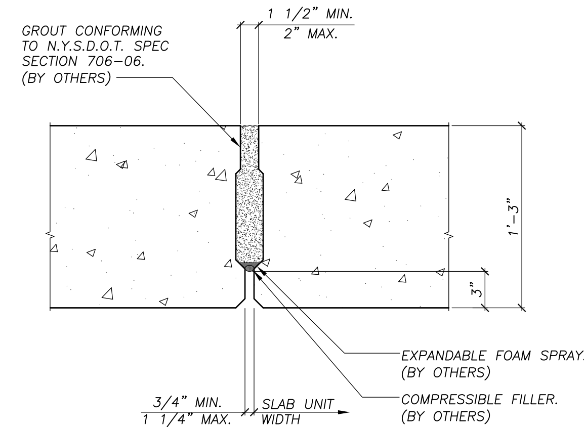
SHEAR KEY DETAIL 1 1/2"=1'-0"
