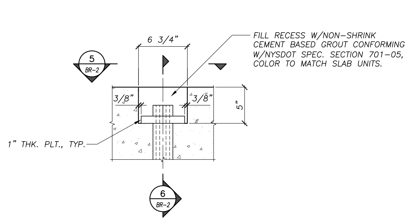
TRANSVERSE TENDON RECESS 1 1/2"=1'-0"
