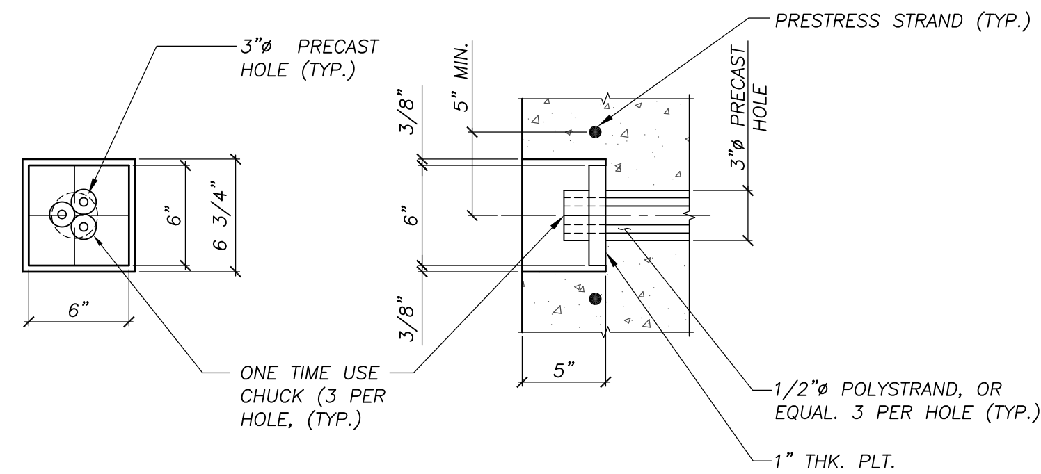
SECTION 5 1 1/2"=1'-0"
