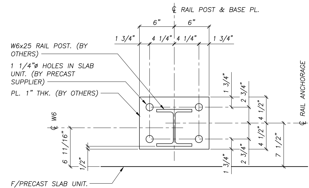
RAIL POST BASE PLATE DETAIL 1 1/2"=1'-0"
