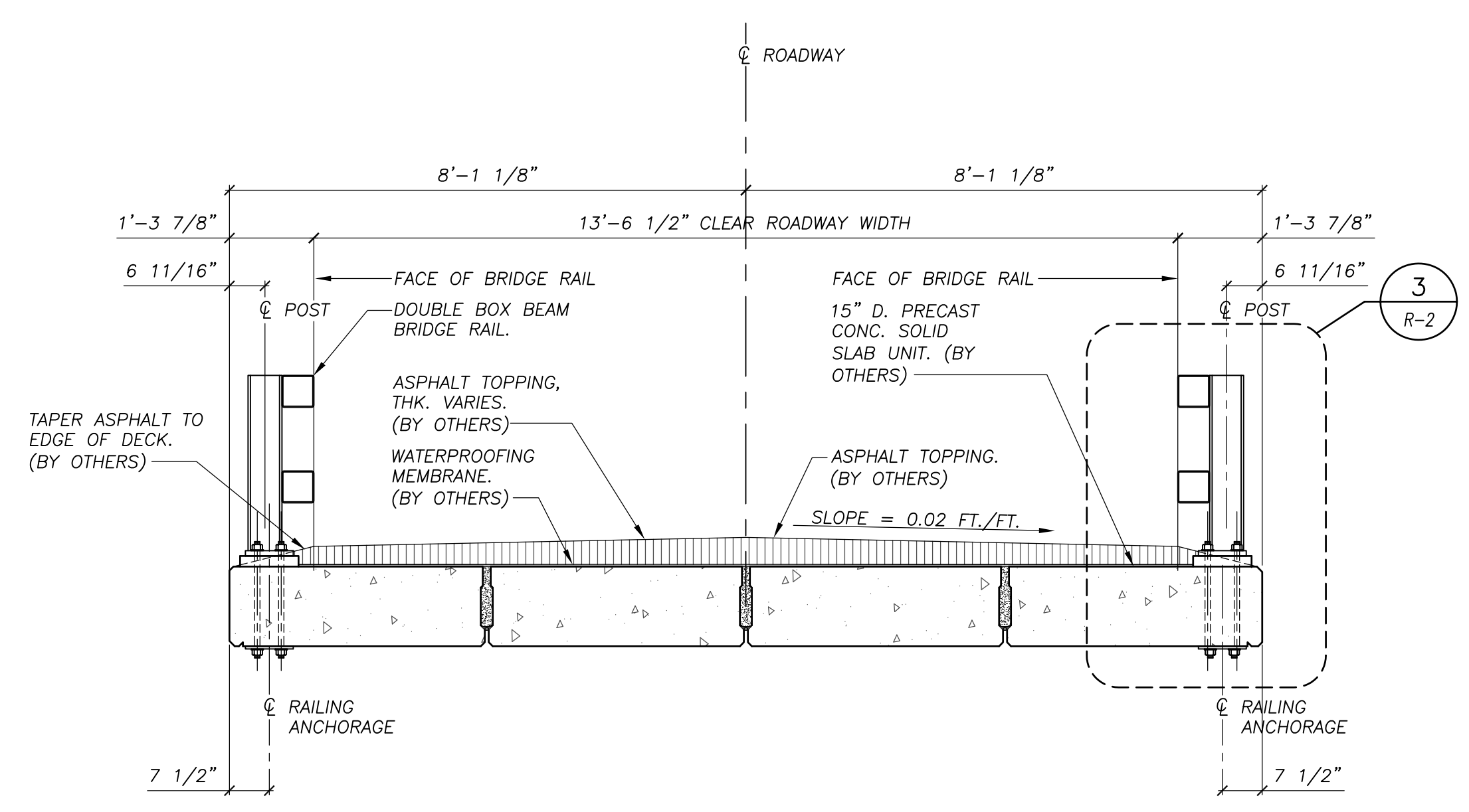
SECTION 2 1/2"=1'-0"
