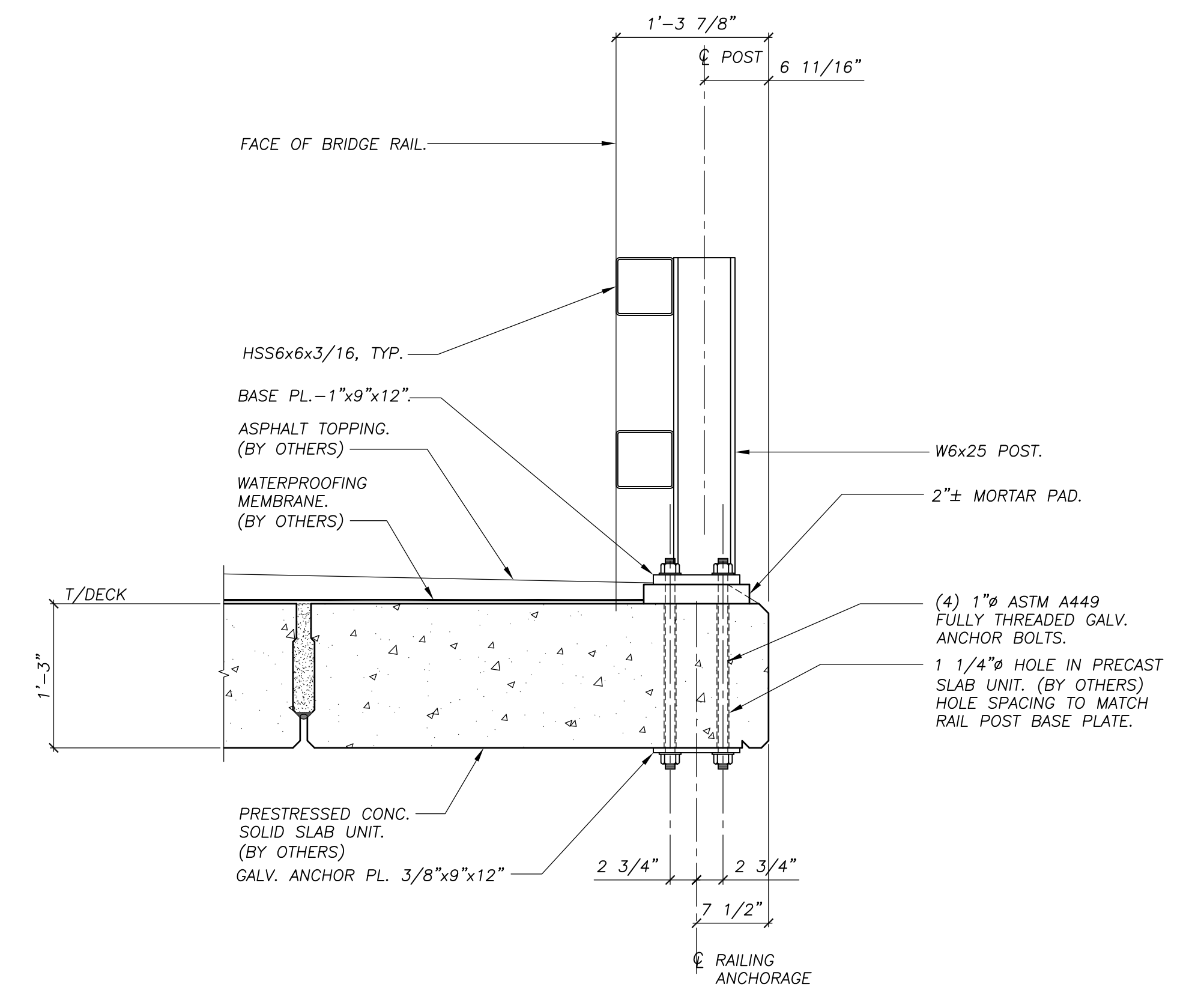
SECTION 3 1"=1'-0"
