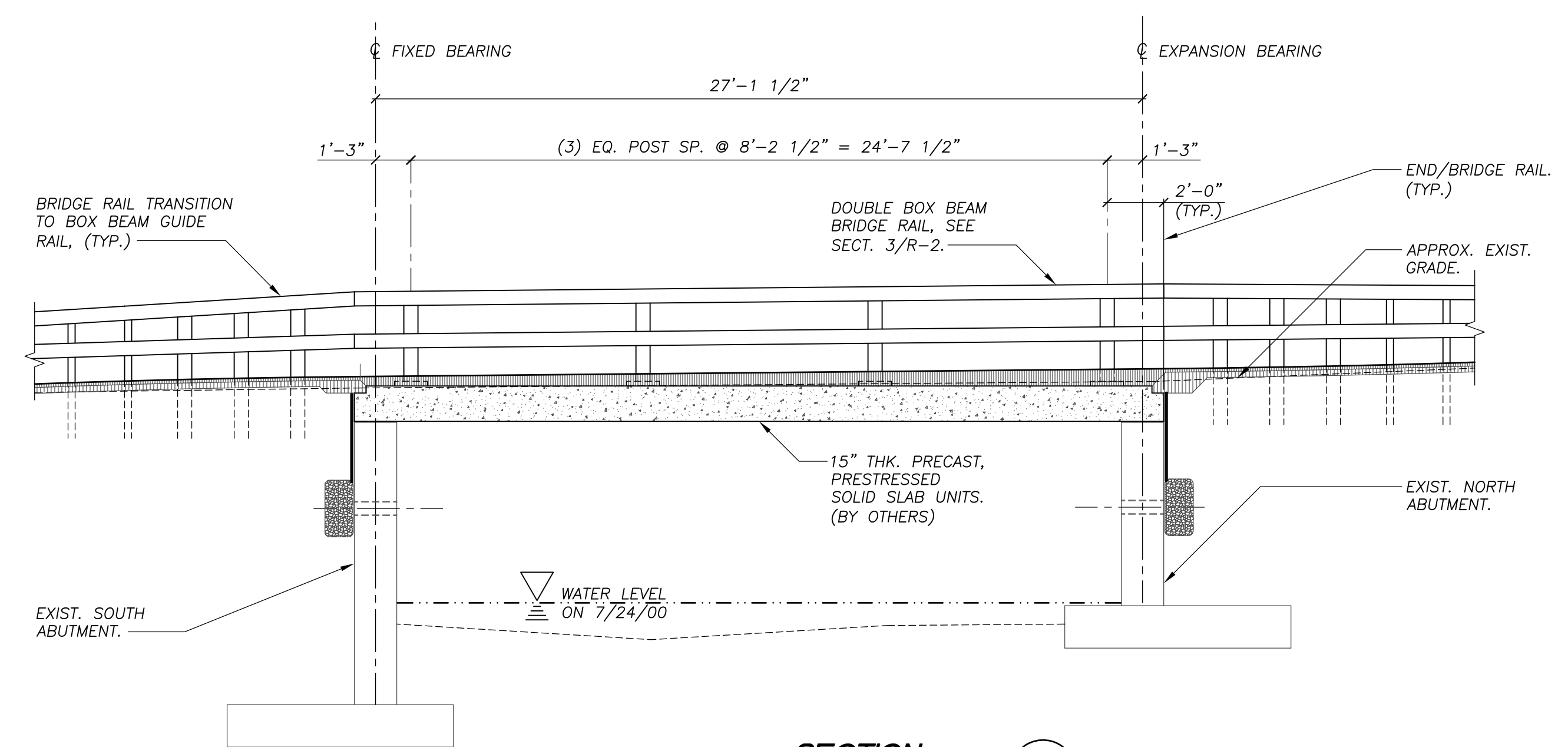
SECTION 1 1/4"=1'-0"
