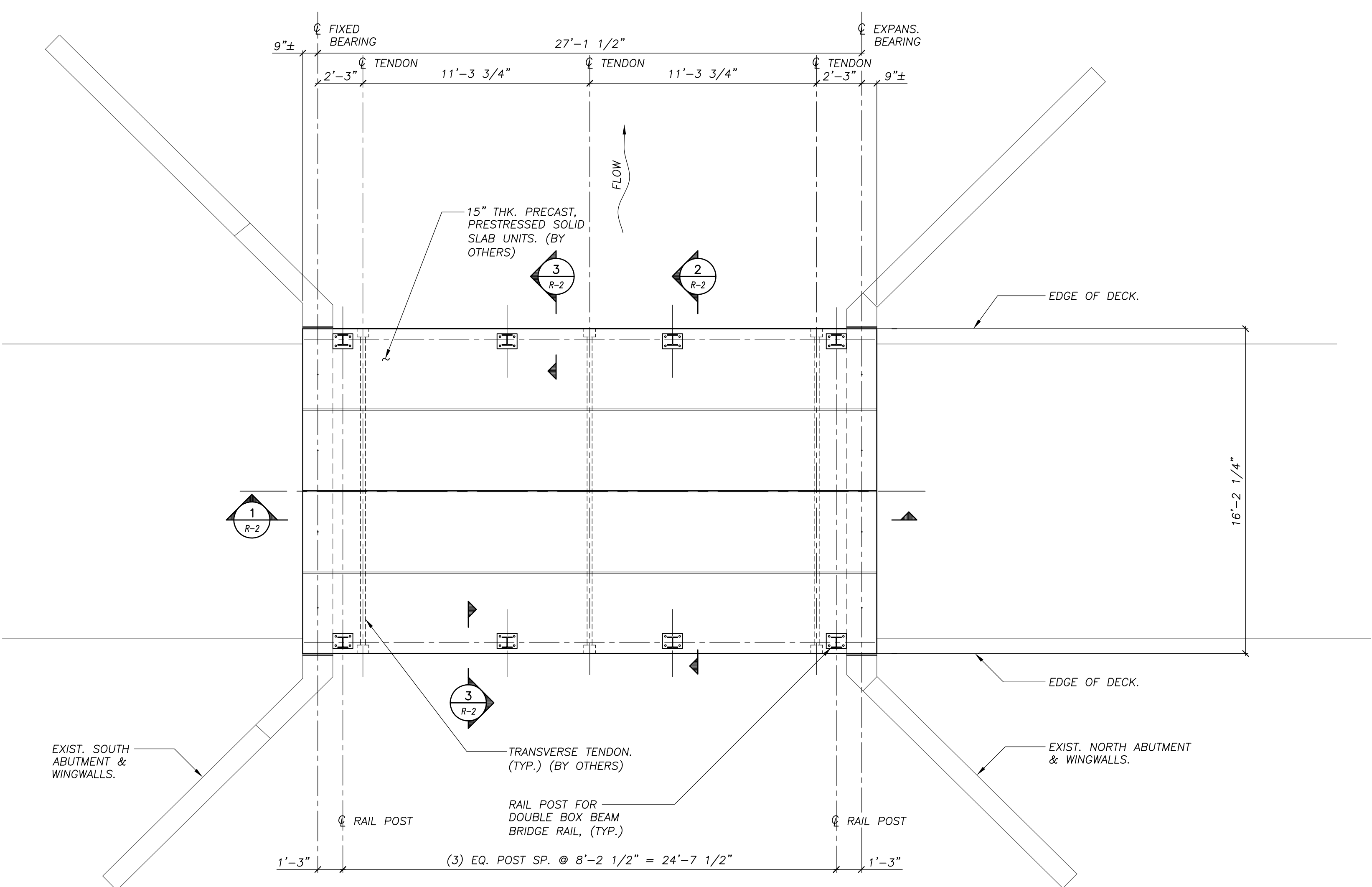
DECK PLAN 1/4"=1'-0"
