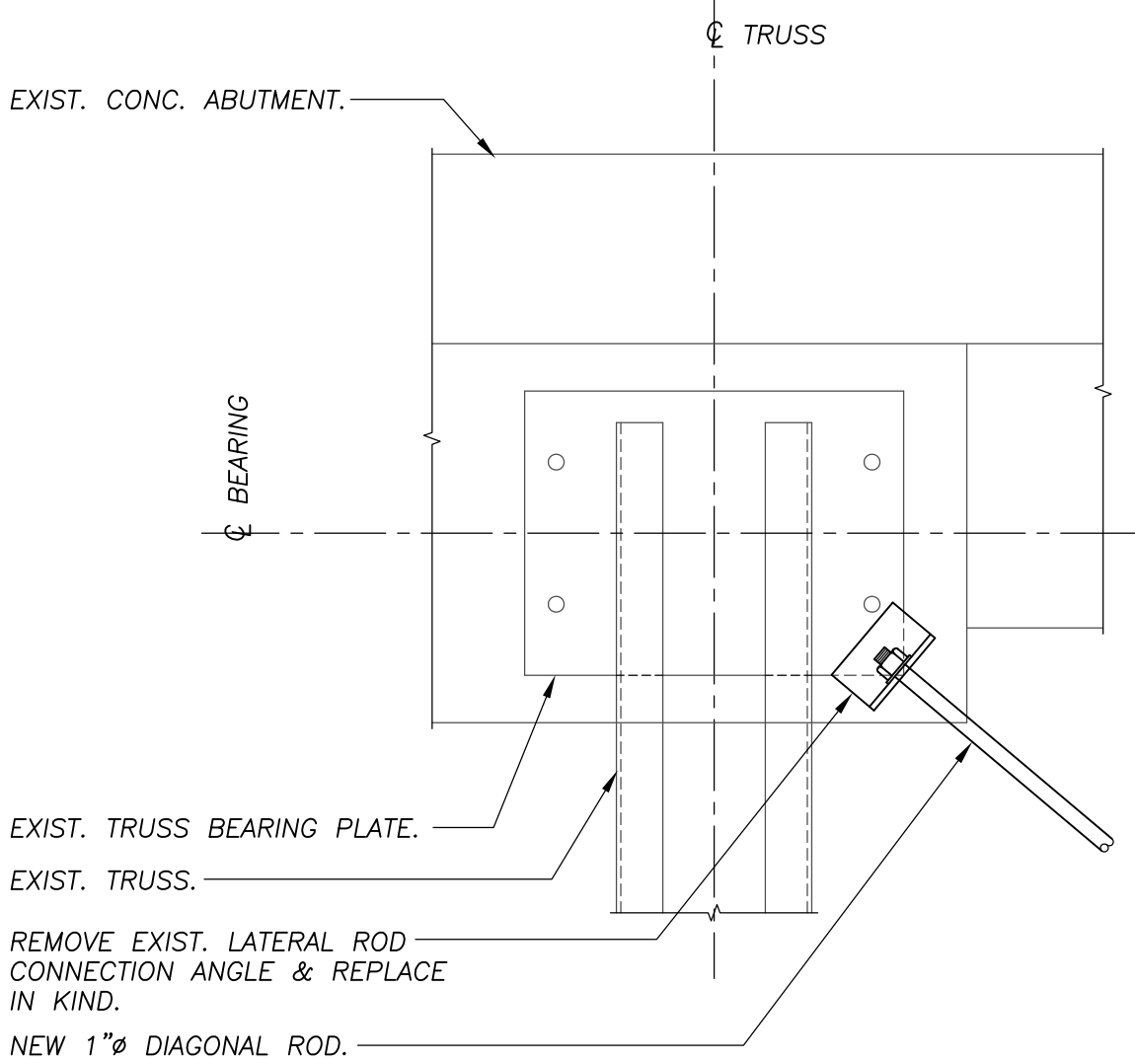
DETAIL A 1"=1'-0"
