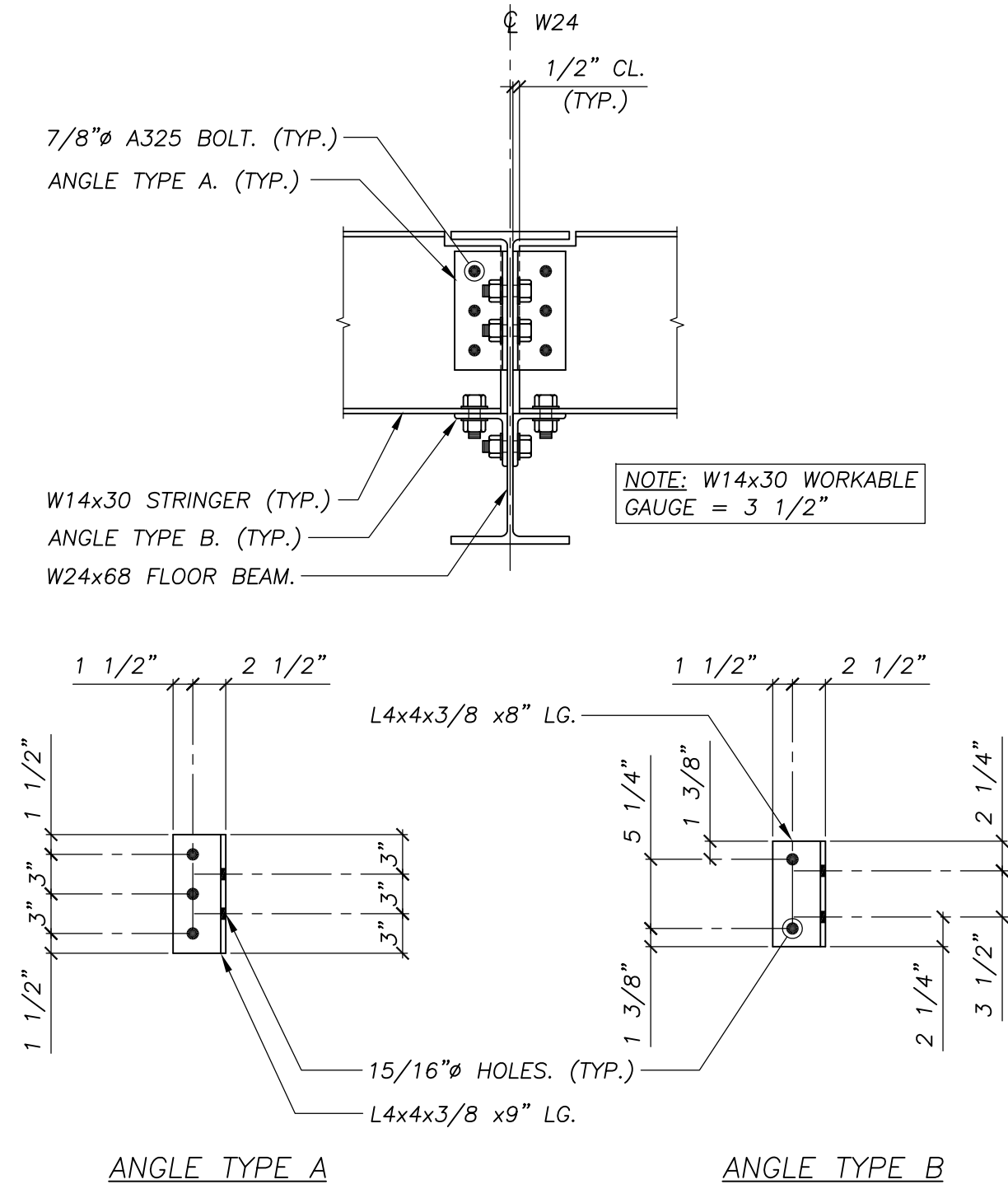
TYPICAL STRINGER CONNECTION DETAIL 1"=1'-0"
