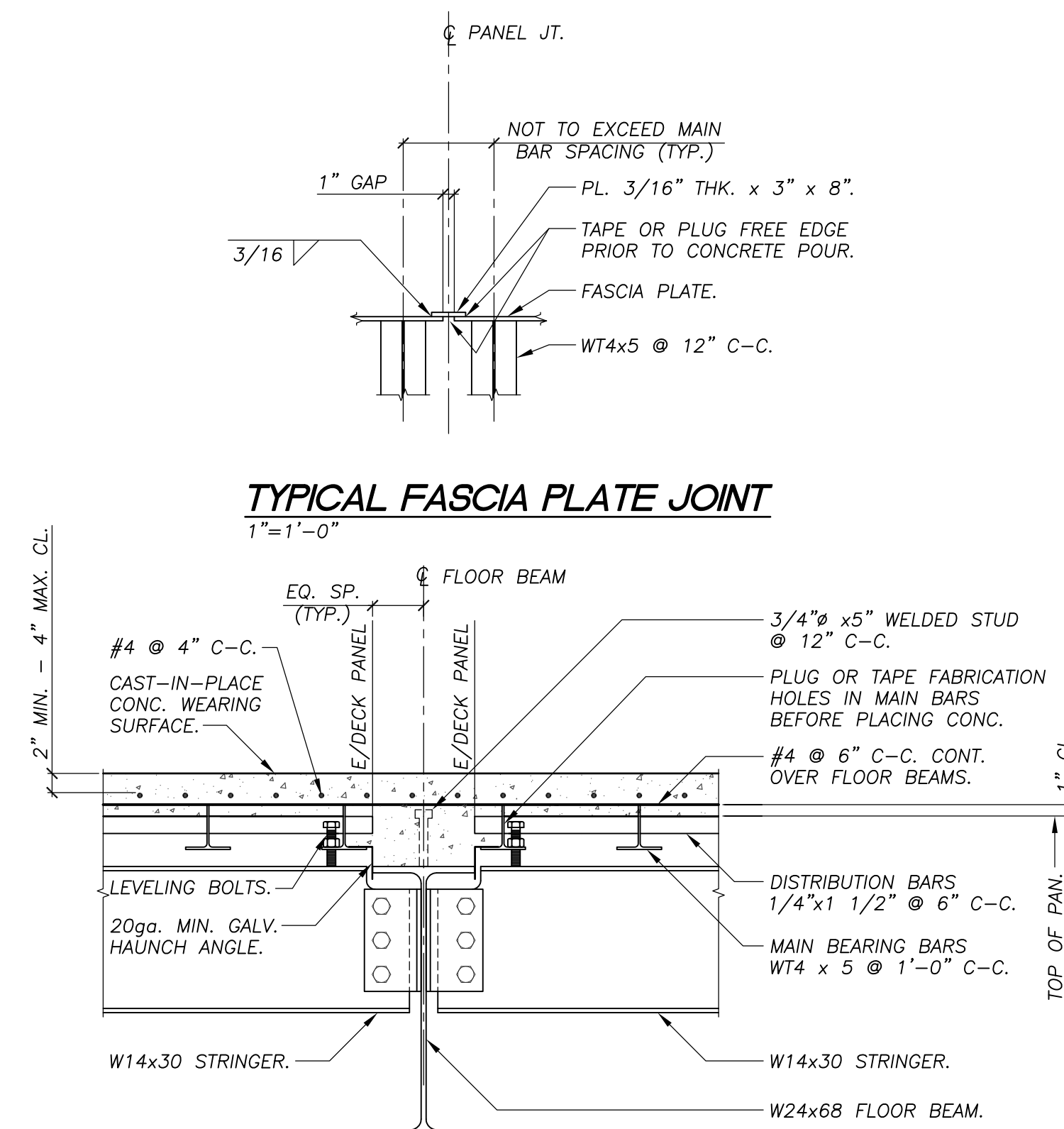
TYPICAL PANEL CONNECTION AT FLOORBEAM DETAIL 1"=1'-0"
