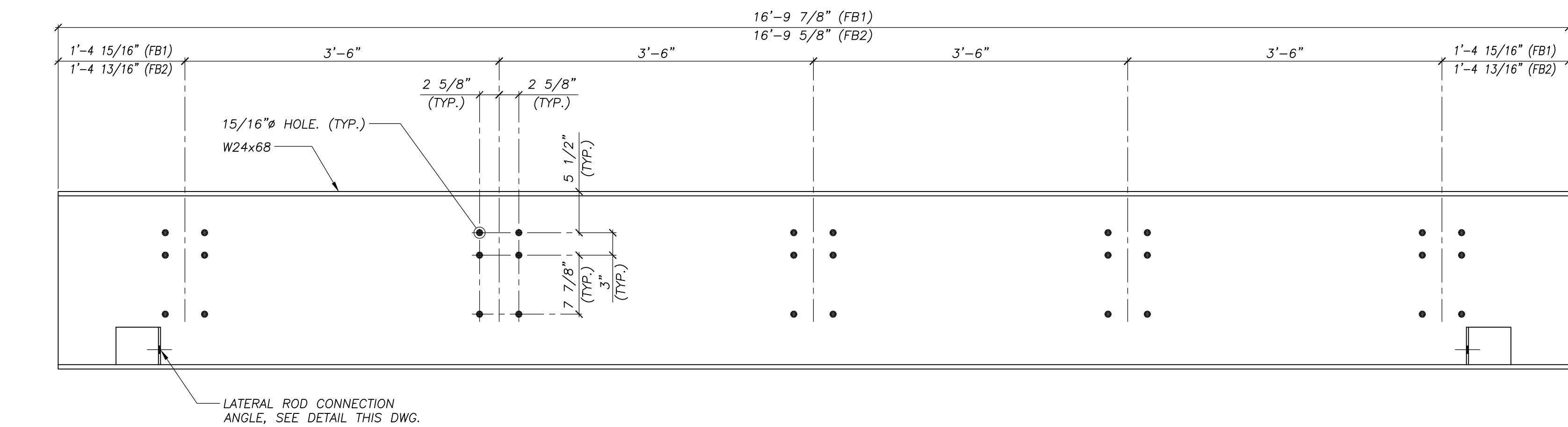
TYPICAL FLOOR BEAM DETAIL 1"=1'-0"
