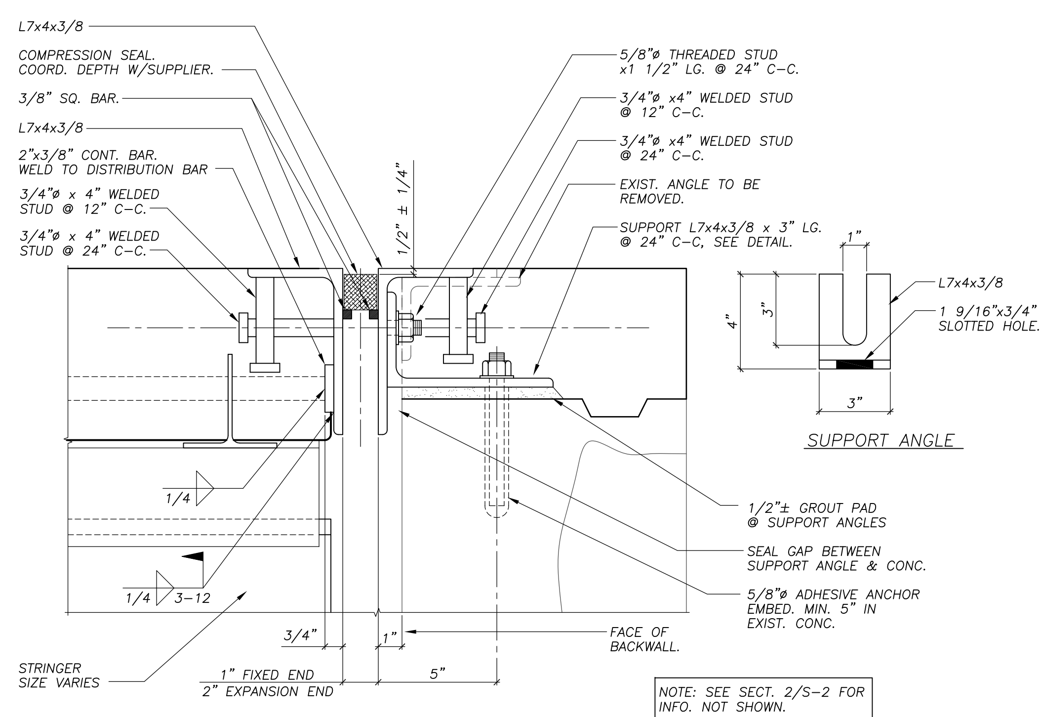
ARMORED JOINT SYSTEM DETAIL 3"=1'-0"
