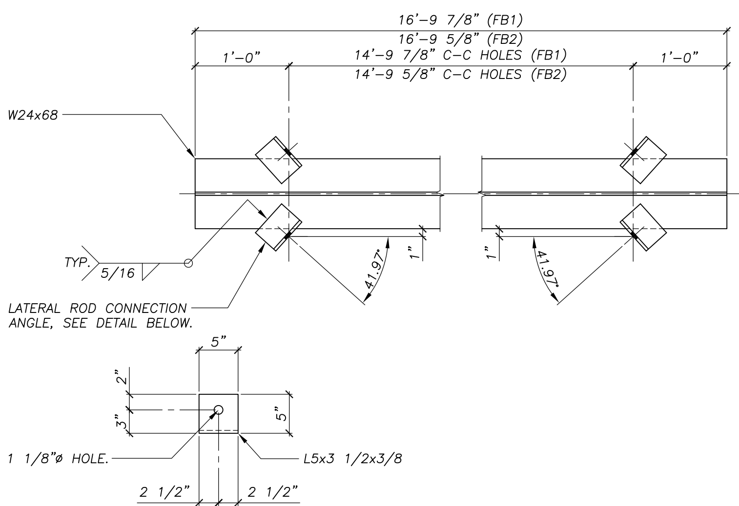
TYPICAL LATERAL ROD CONNECTION ANGLE DETAIL 1"=1'-0"
