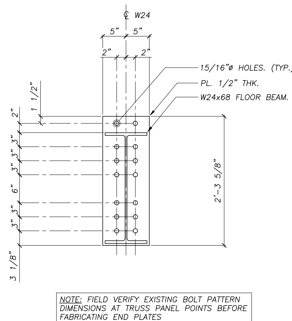
TYPICAL FLOOR BEAM END PLATE DETAIL 1"=1'-0"
