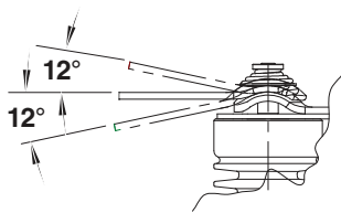
HINGE TERMINAL PAD ARTICULATING DETAIL
