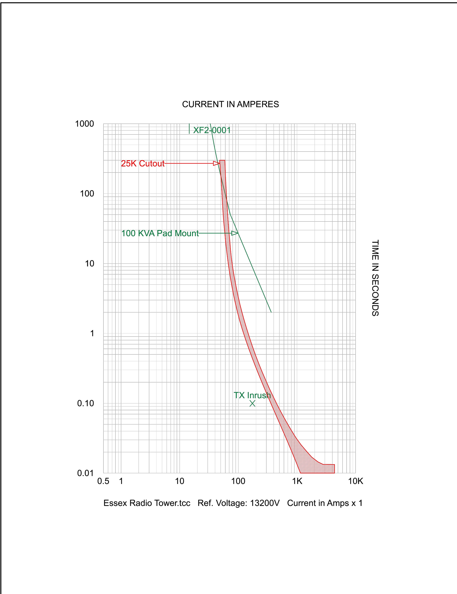
FUSE LINK VS. TRANSFORMER INRUSH AND DAMAGE CURVE.
