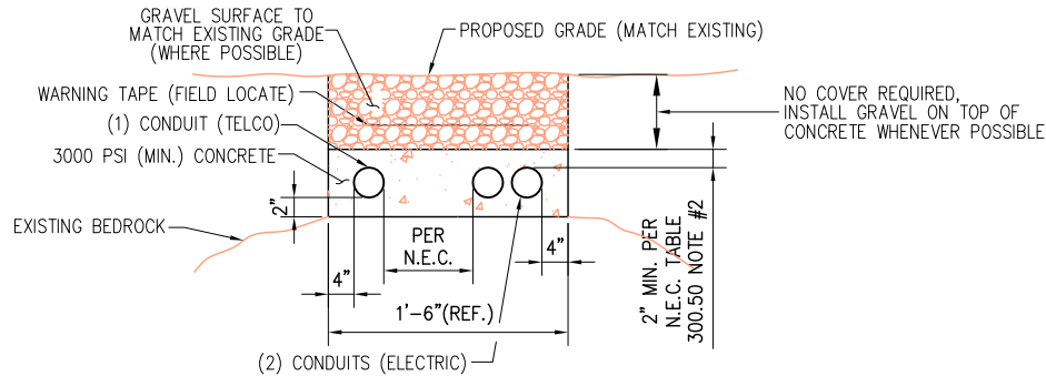
2 CONCRETE ENCASEMENT CONDUIT TRENCH DETAIL NOT TO SCALE
