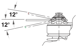
HINGE TERMINAL PAD ARTICULATING DETAIL
