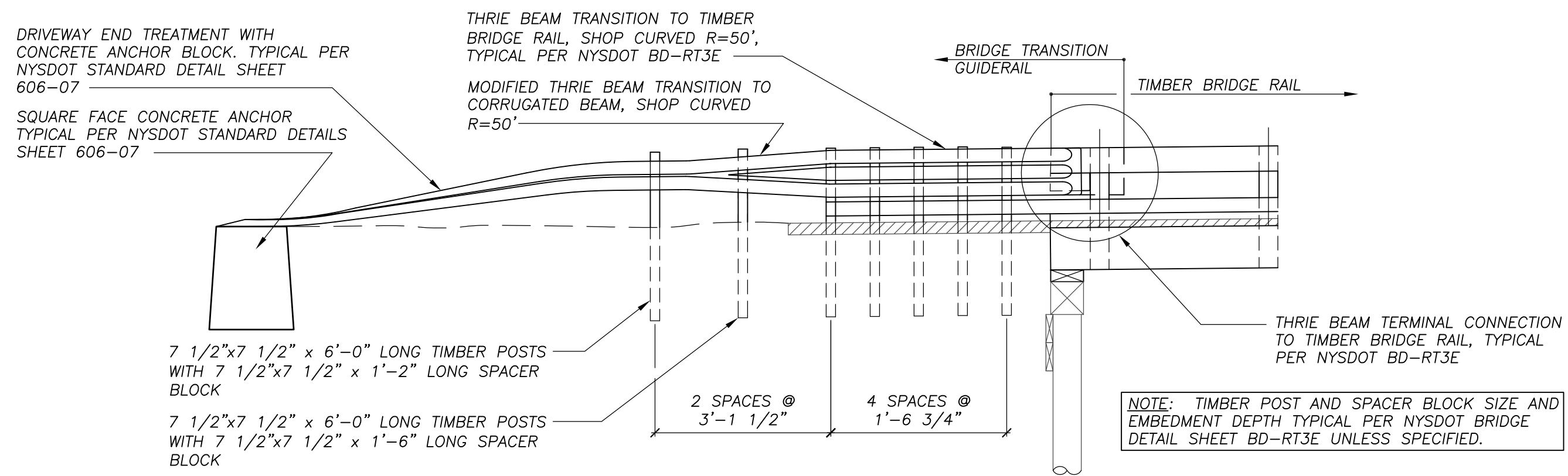
MODIFIED THRIE BEAM TRANSITION TO CORRUGATED BEAM 1/4"=1'-0"
