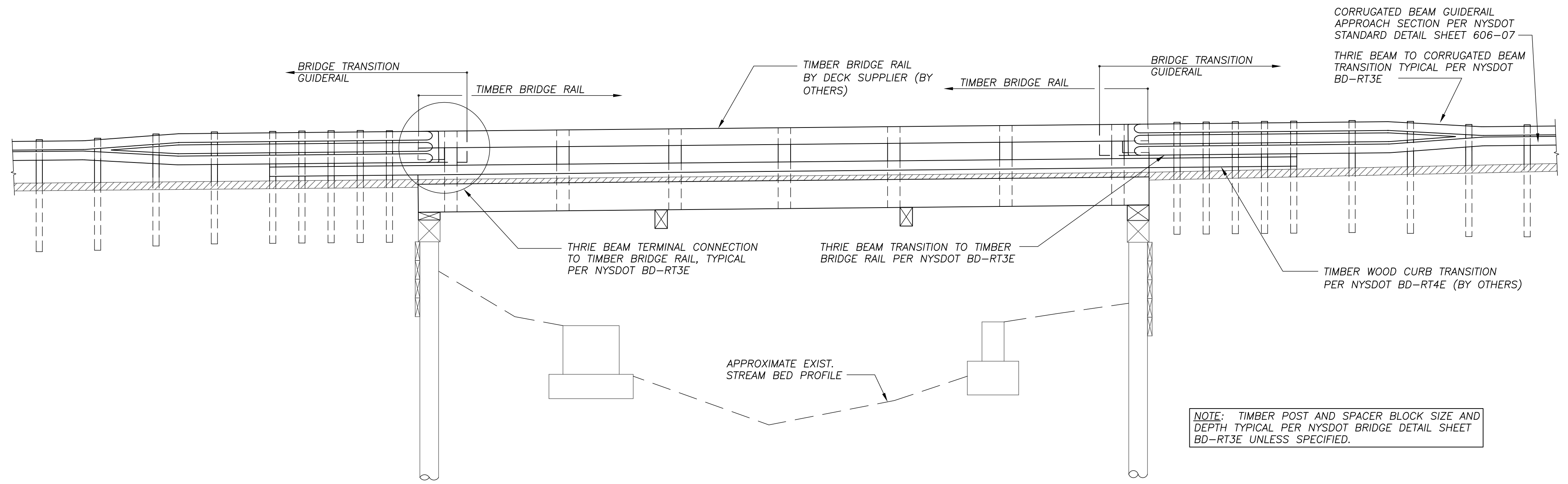
GUIDERAIL ELEVATION 1/4"=1'-0"
