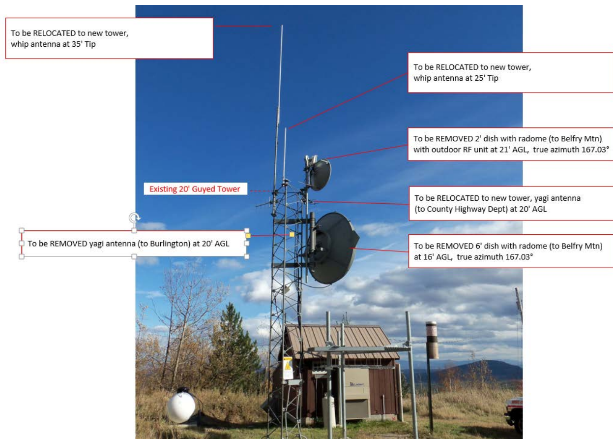
Figure 3 – Wells Hill tower profile
