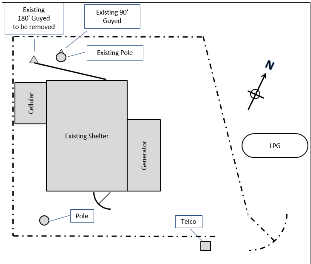
Figure 1 – Belfry Mountain site sketch
