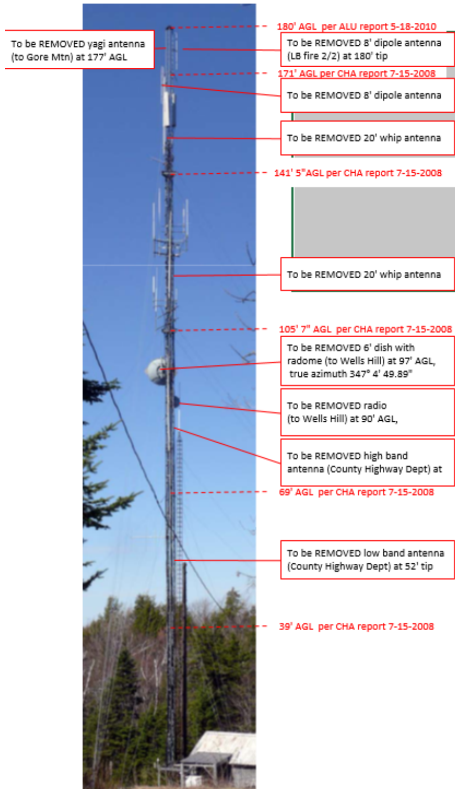
Figure 2 – Belfry Mountain tower profile
