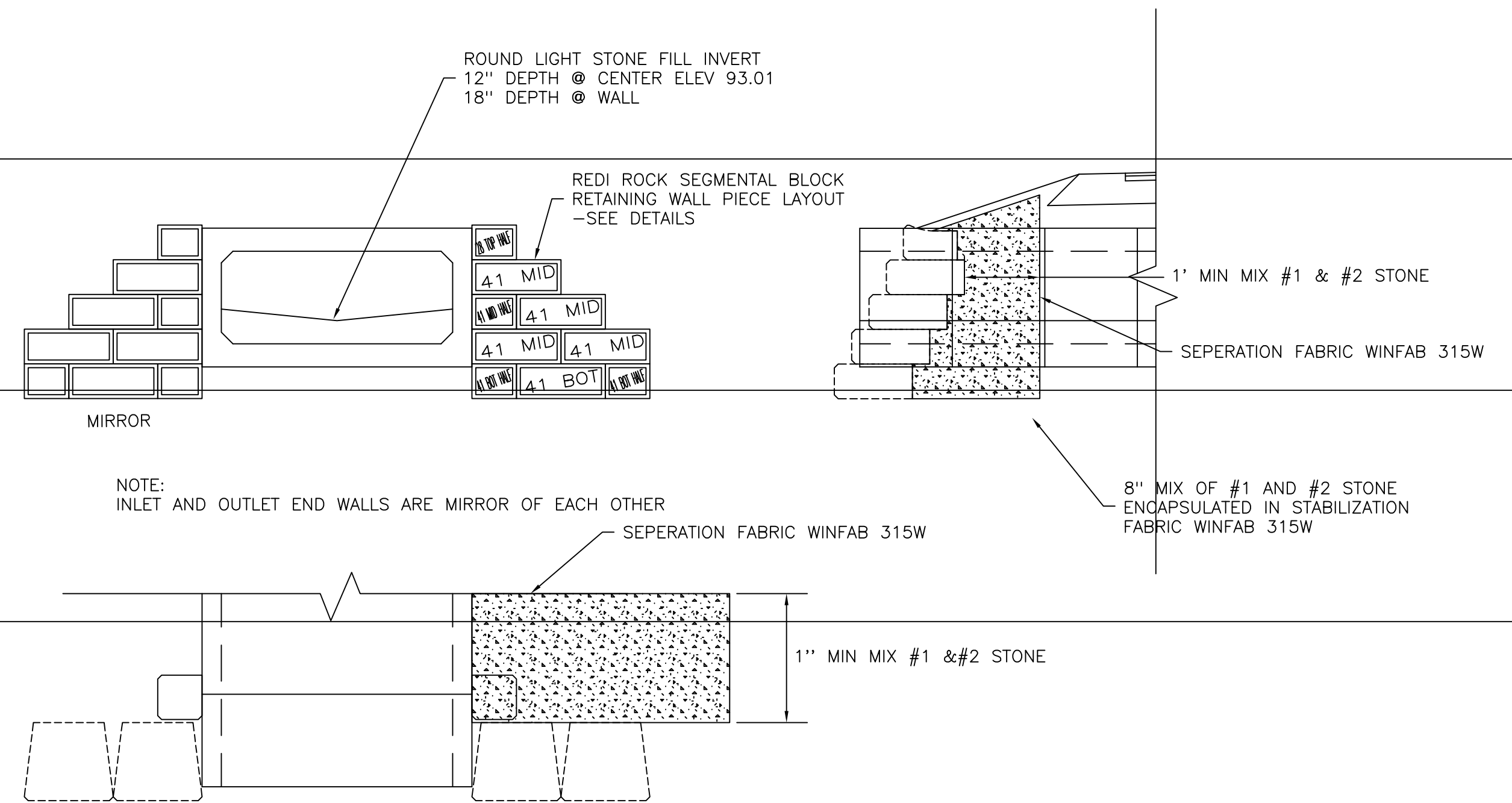
SEGMENTAL BLOCK RETAINING WALL DETAIL SCALE:1"=5'
