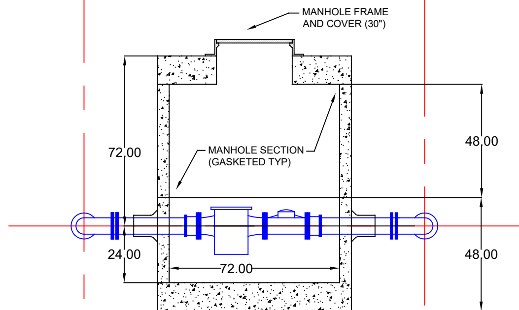
MANHOLE (SECTION)
