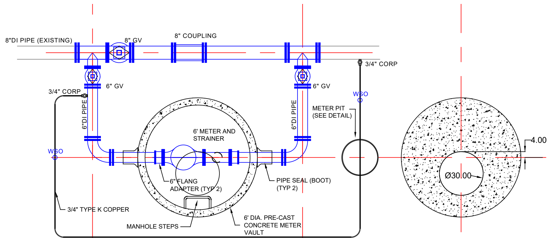
MANHOLE (PLAN)
