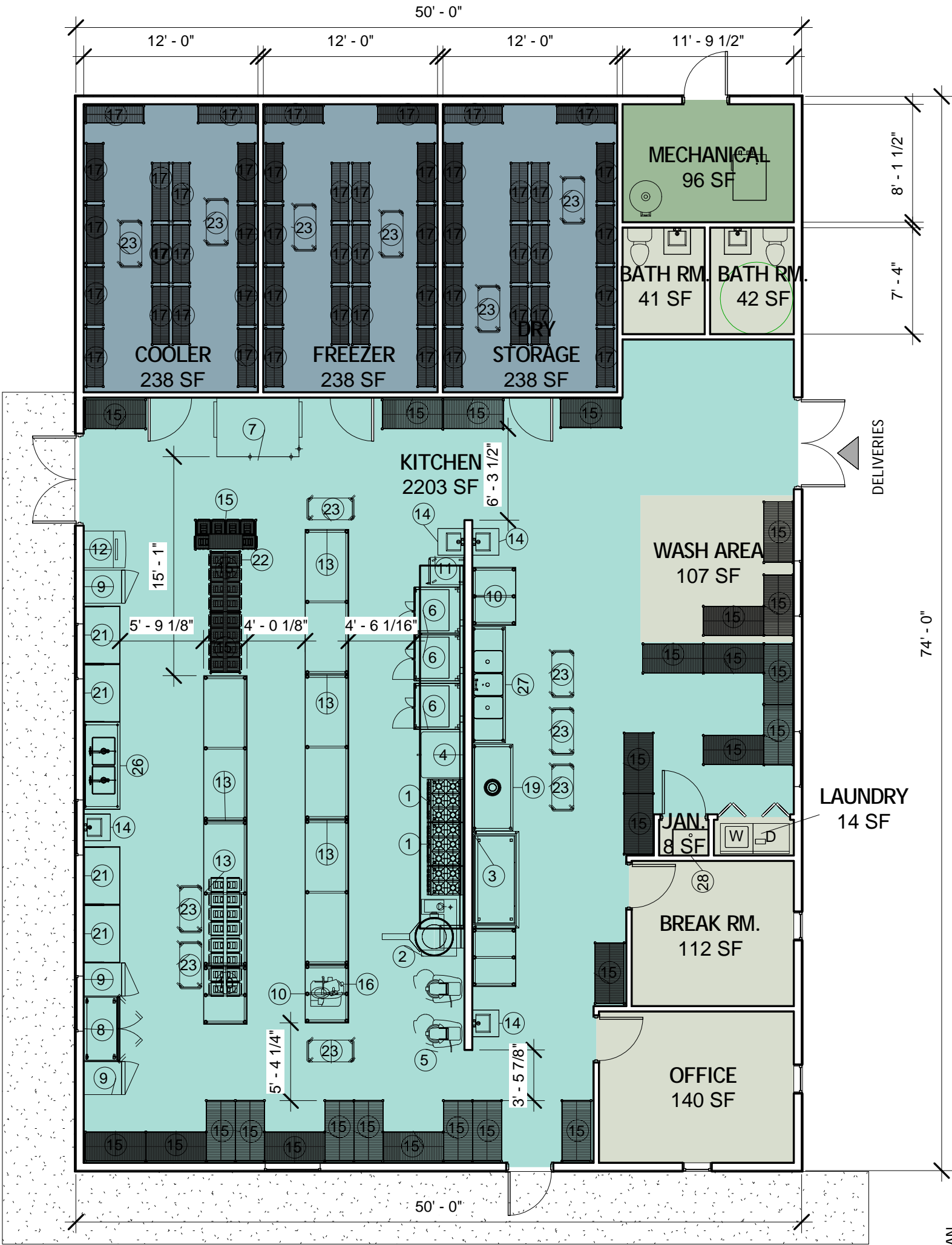
1 FIRST FLOOR PLAN - OPTION B 1/8" = 1'-0"
