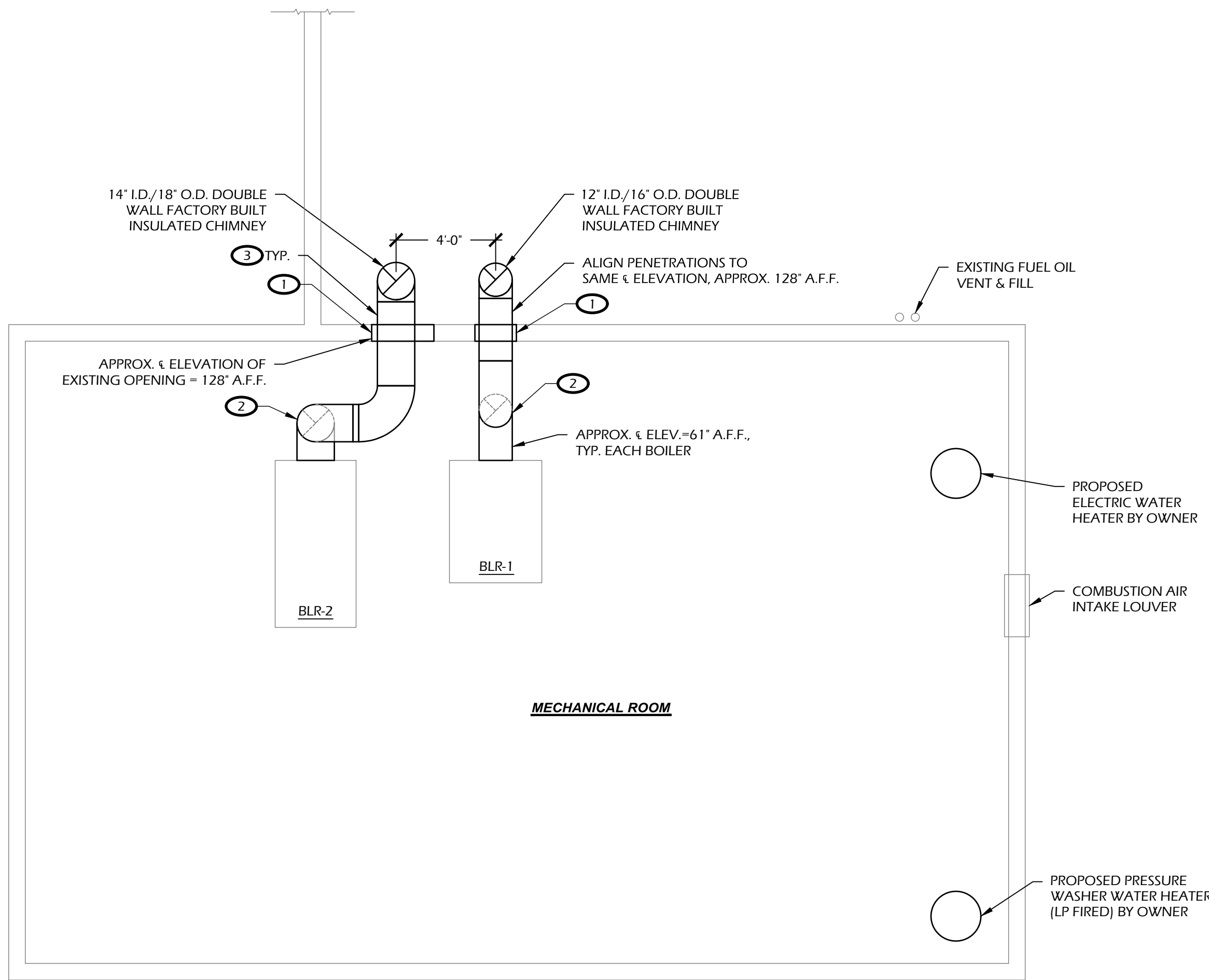
1 MECHANICAL PLAN SCALE: 1/4" = 1'-0"
