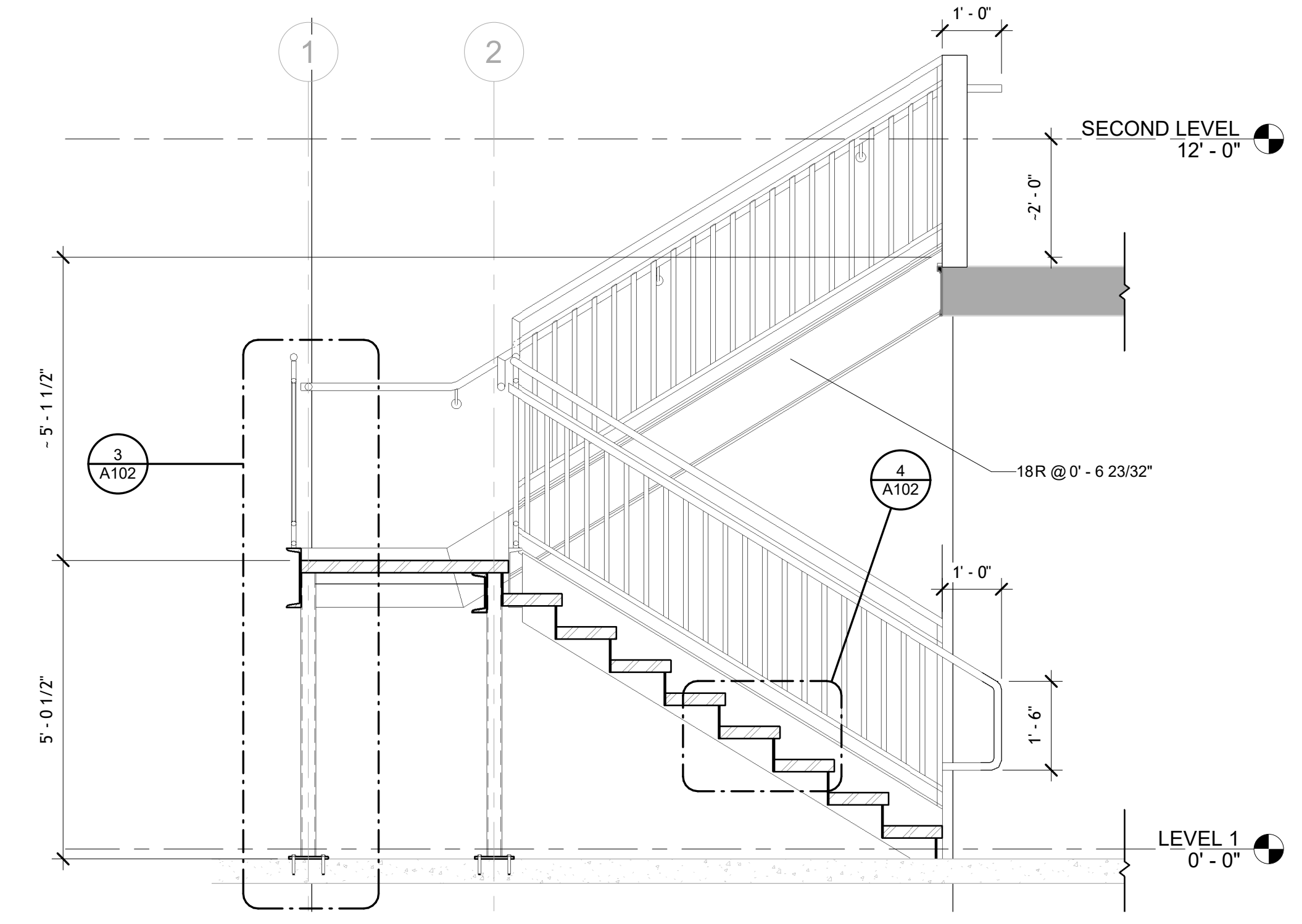
SECTION 3 1/2" = 1'-0"
