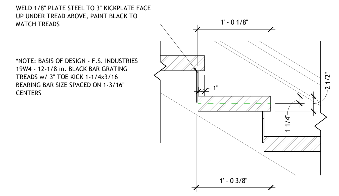
TREAD DETAIL 1 1/2" = 1'-0"
