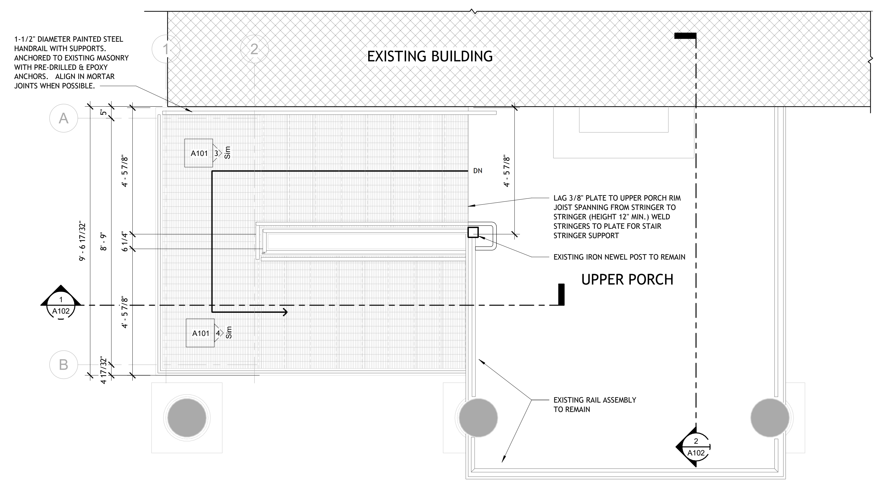
2 SECOND LEVEL 1/2" = 1'-0"
