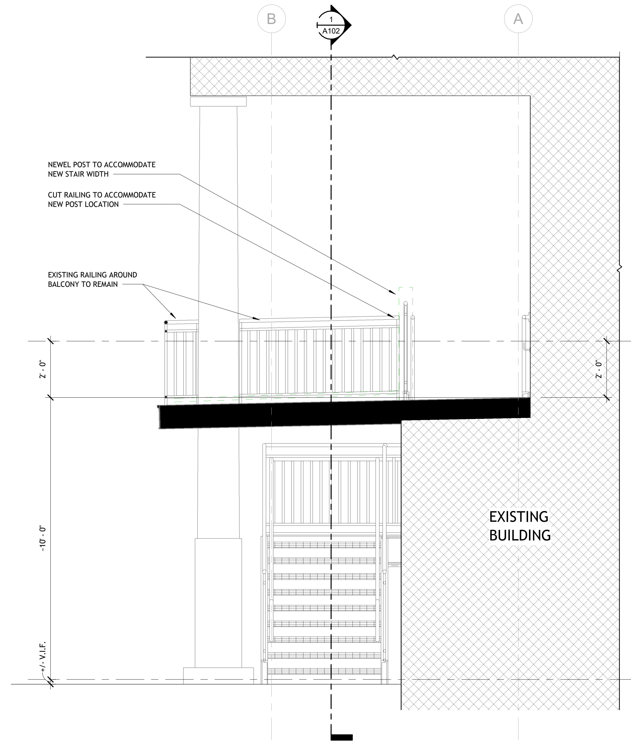
SECTION 1 1/2" = 1'-0"
