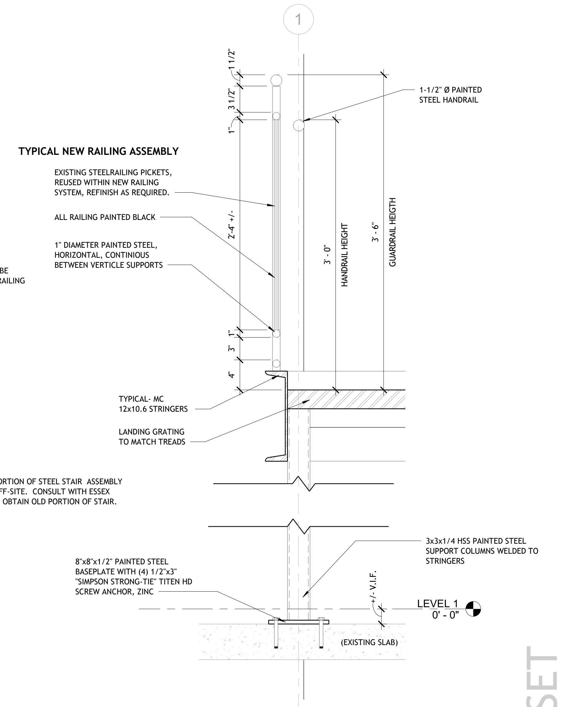
LANDING SUPPORT DETAIL 1 1/2" = 1'-0"
