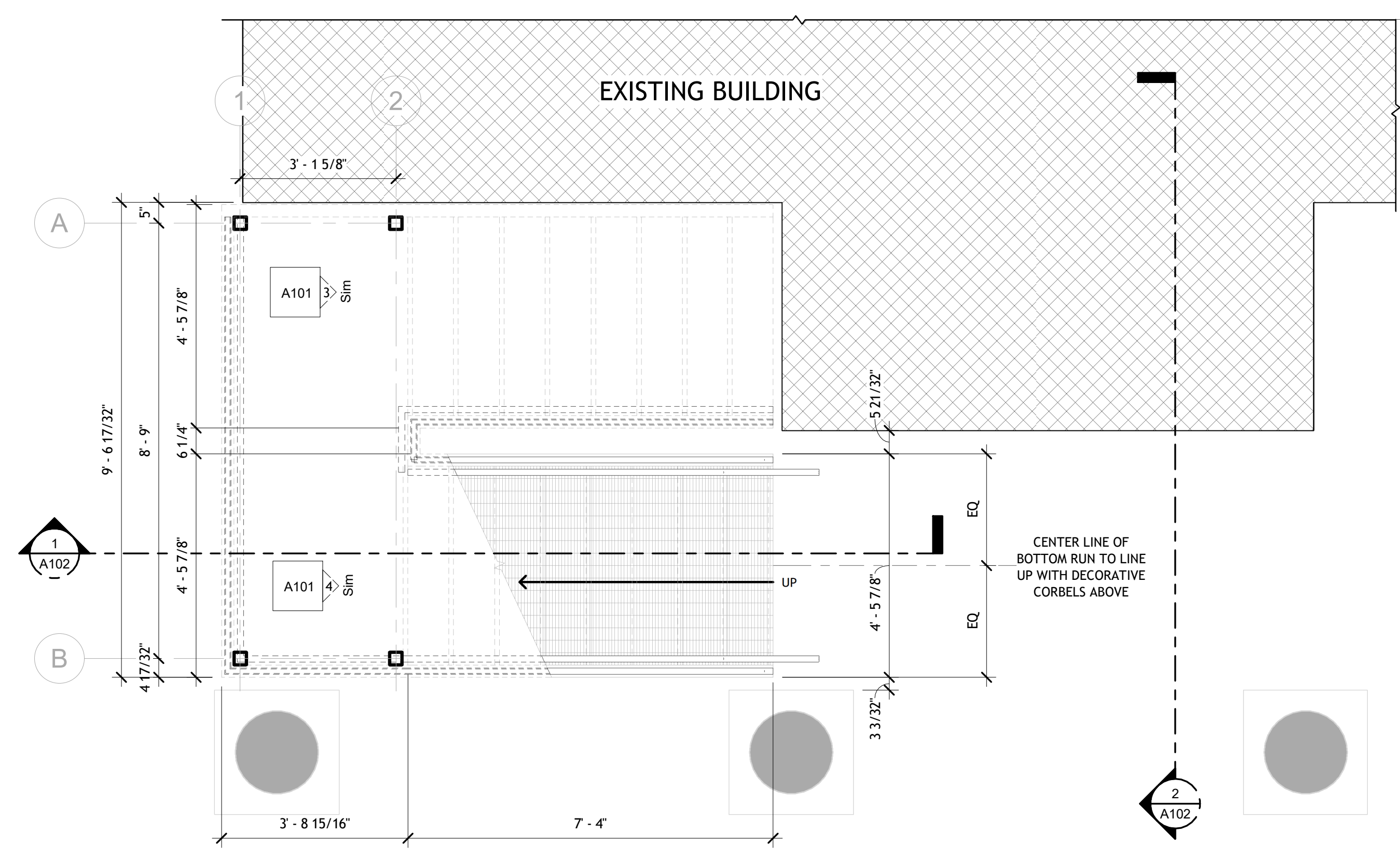
1 GROUND LEVEL 1/2" = 1'-0"
