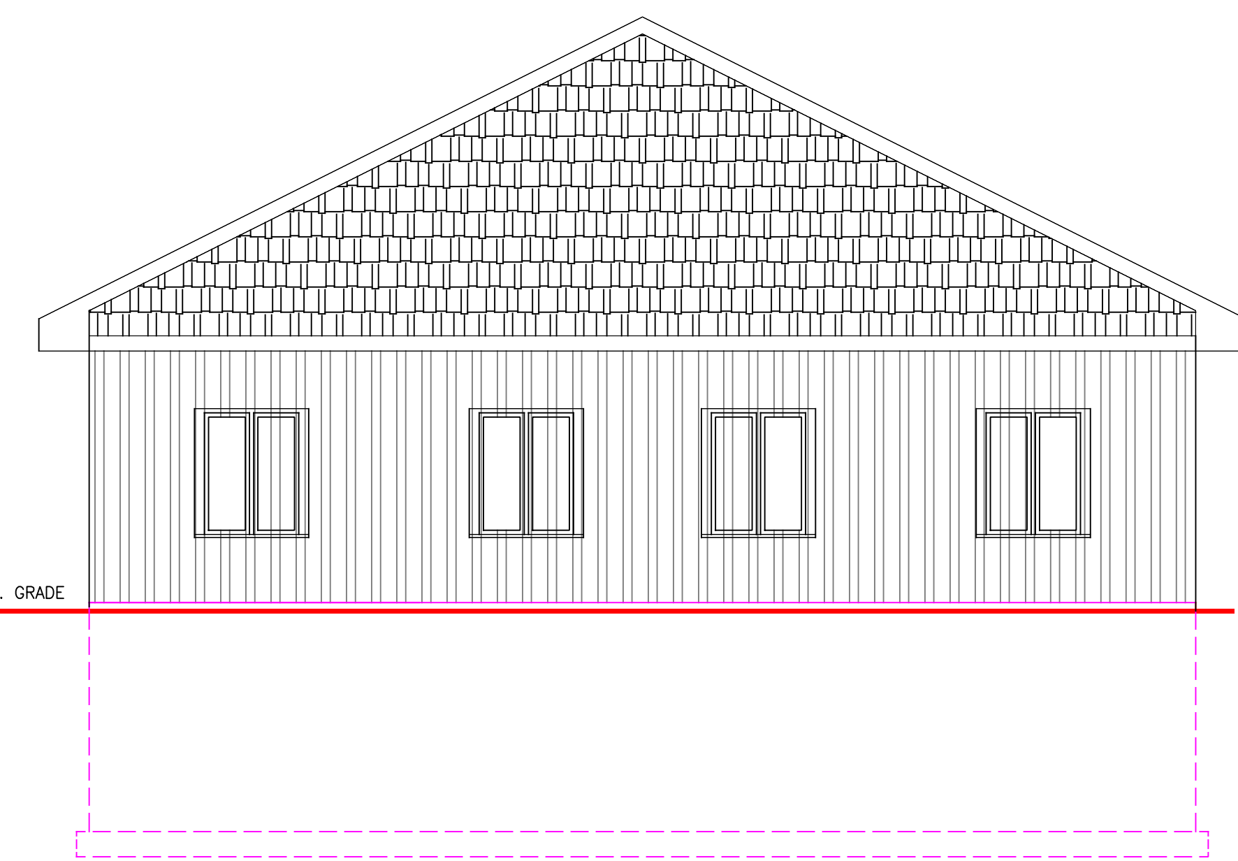
ADDITION ELEVATION (EAST)
