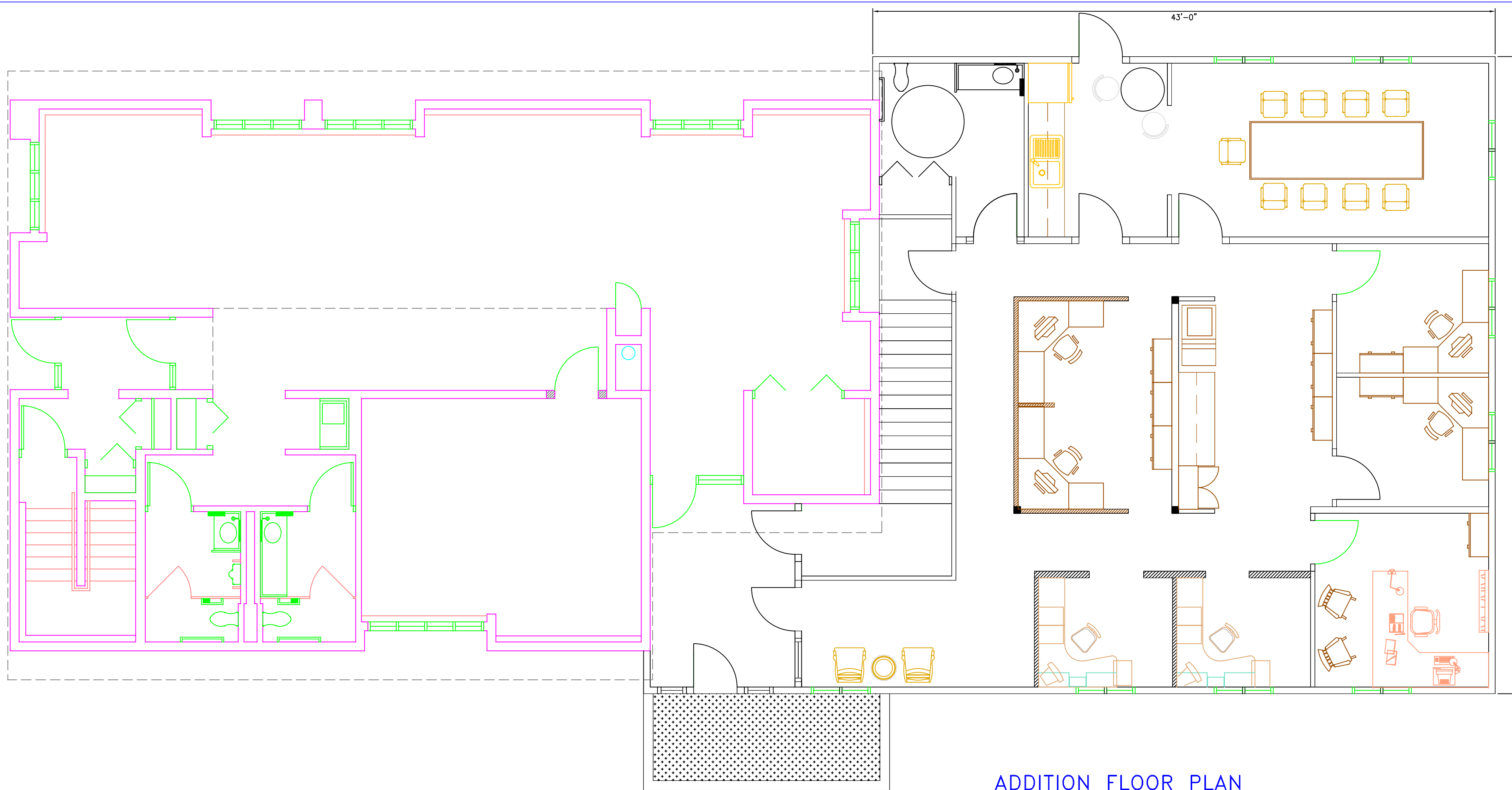
ADDITION FLOOR PLAN
