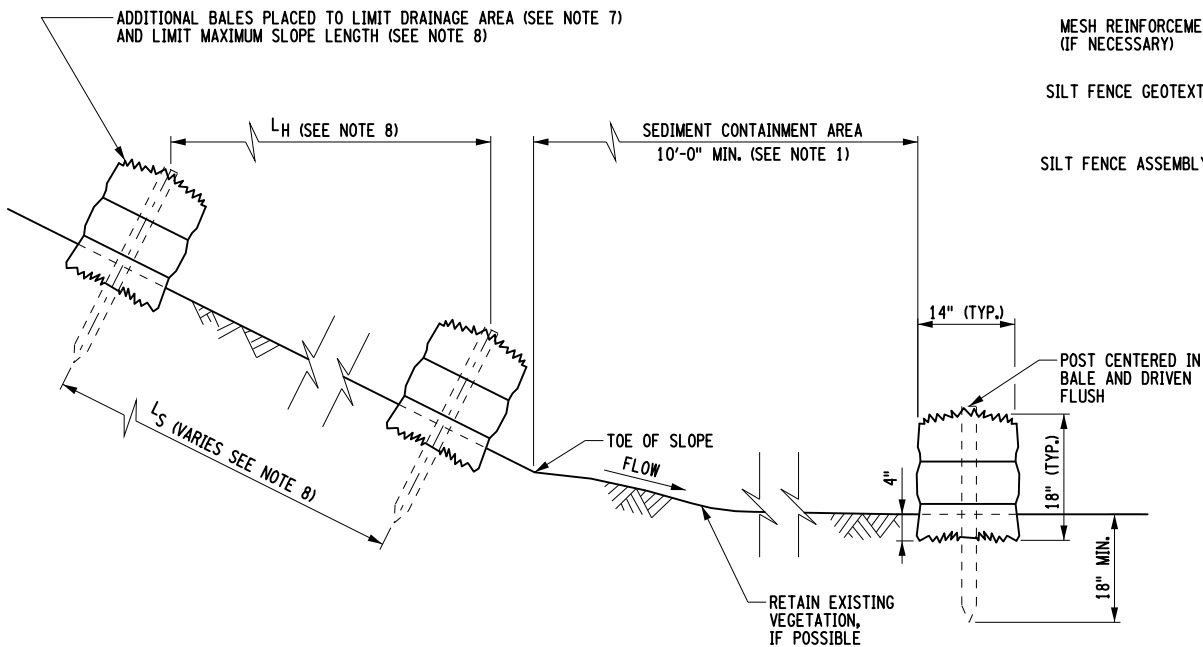
SECTION STRAWBALE DIKE - TEMPORARY
