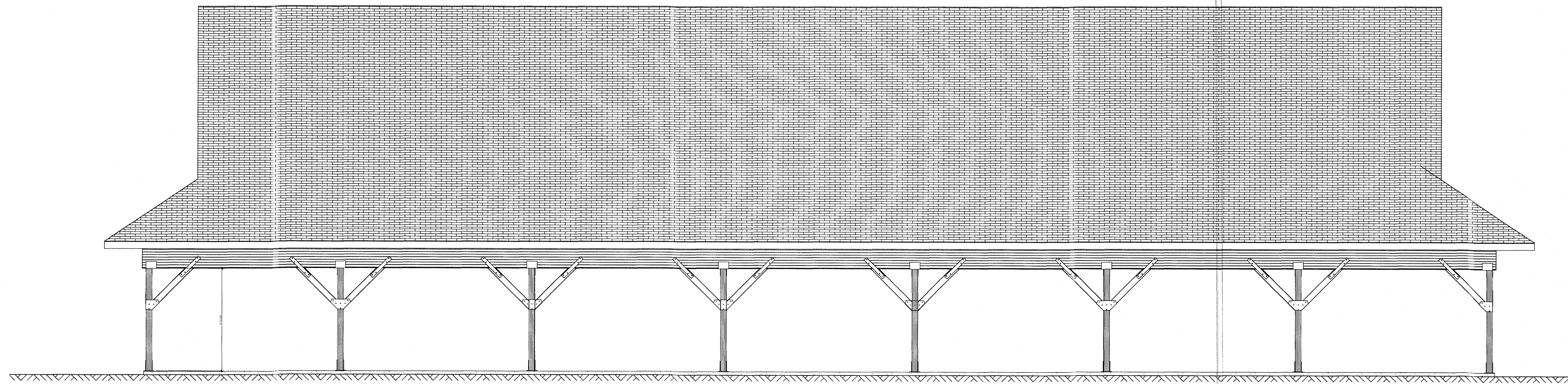
1 NORTH ELEVATION SCALE: 3/16" = 1'-0"
