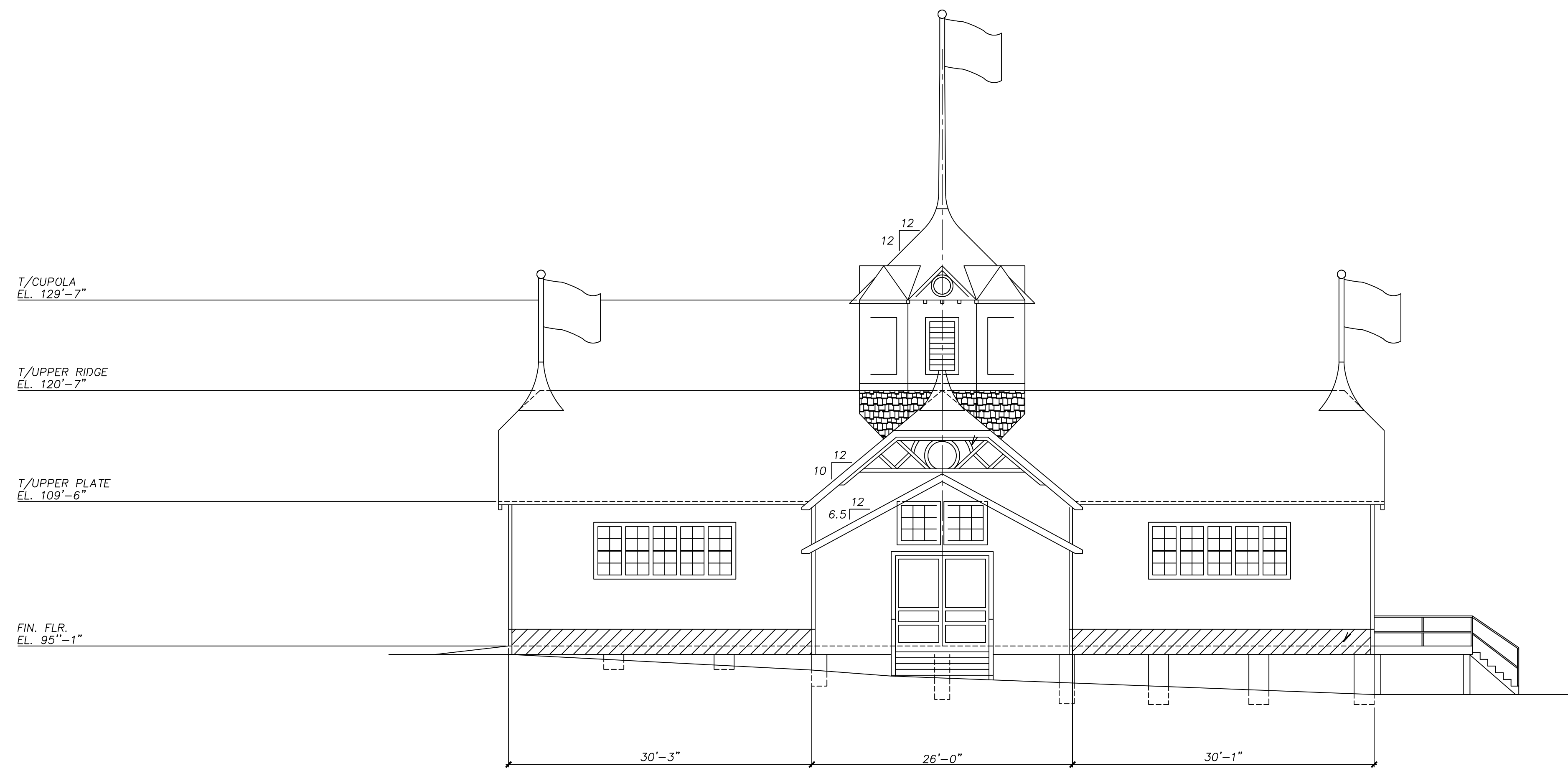
EAST ELEVATION
