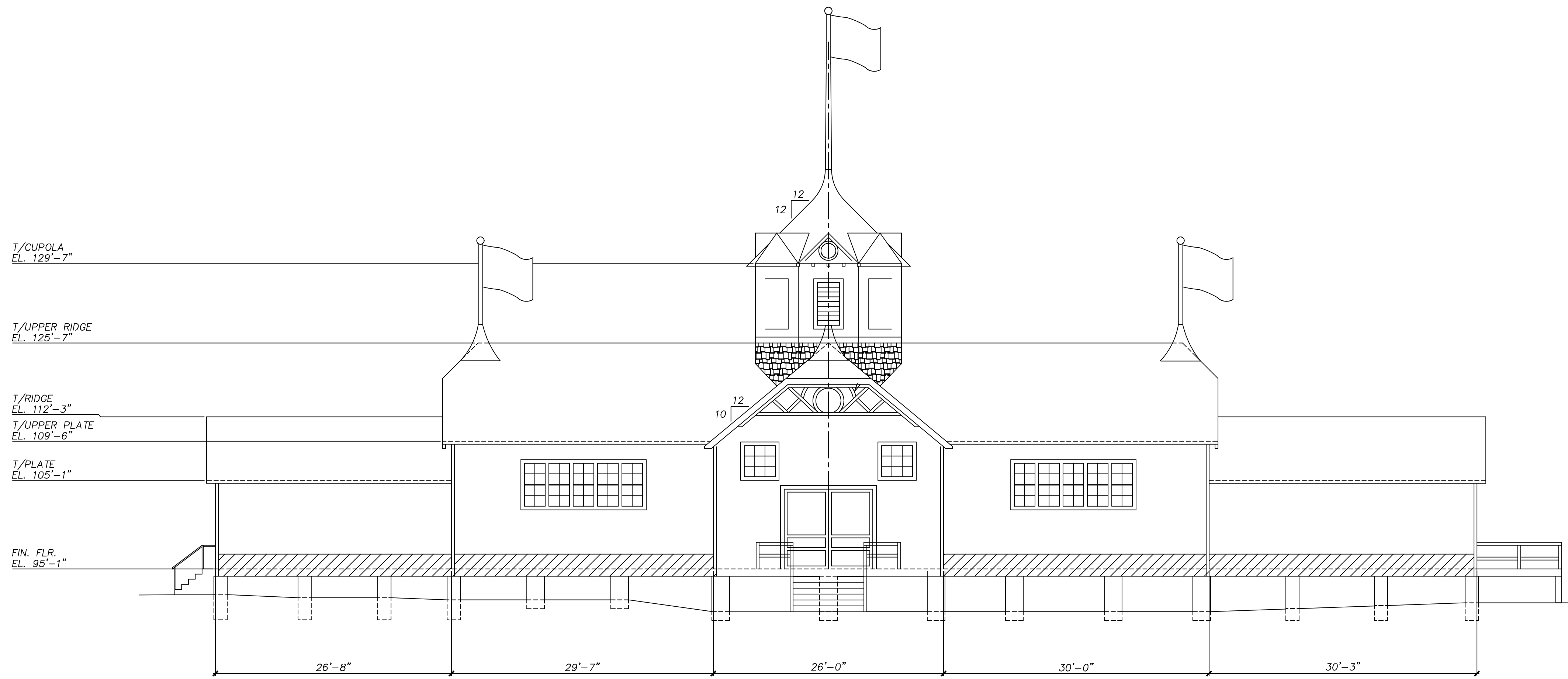
NORTH ELEVATION
