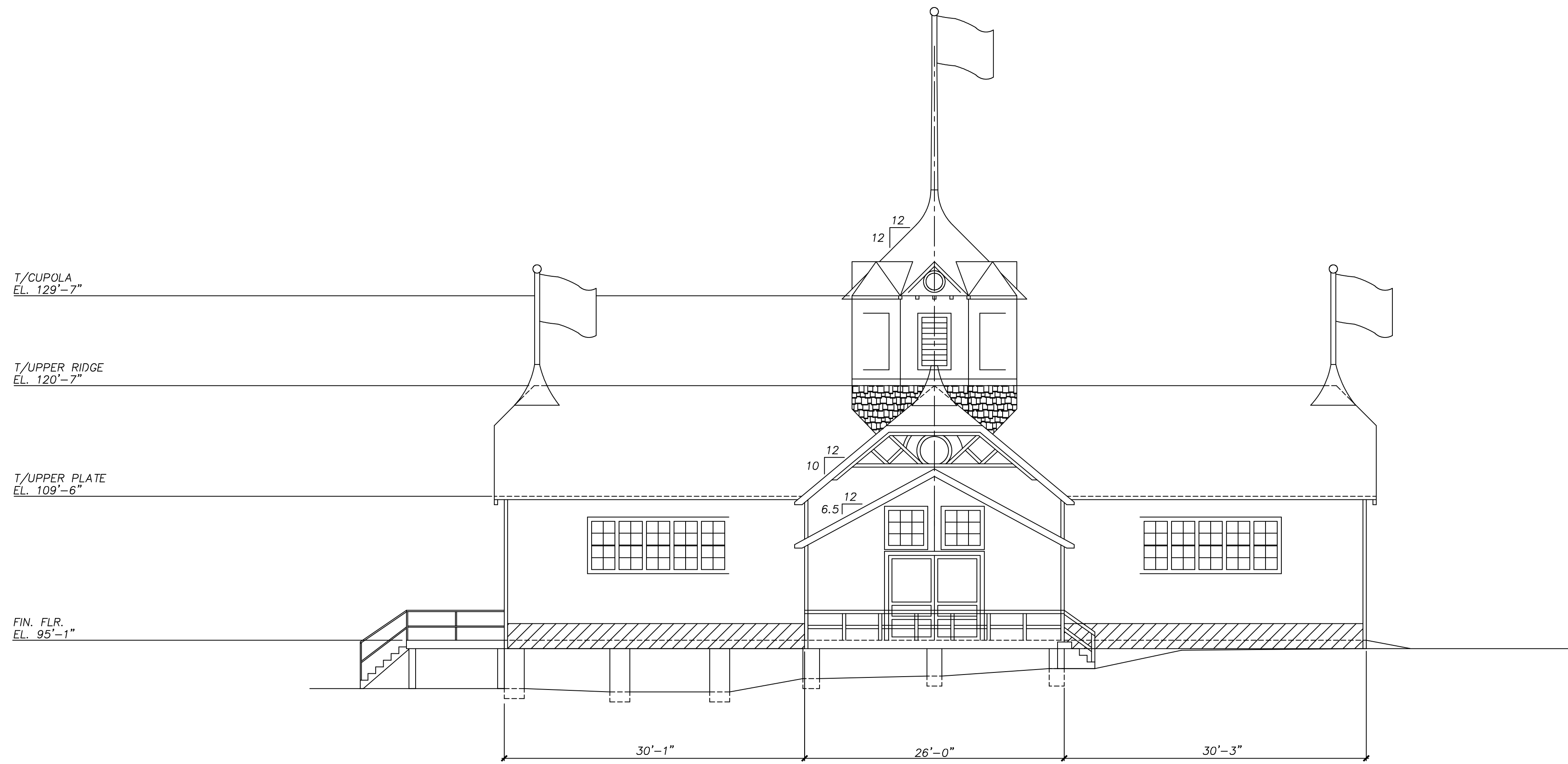
WEST ELEVATION
