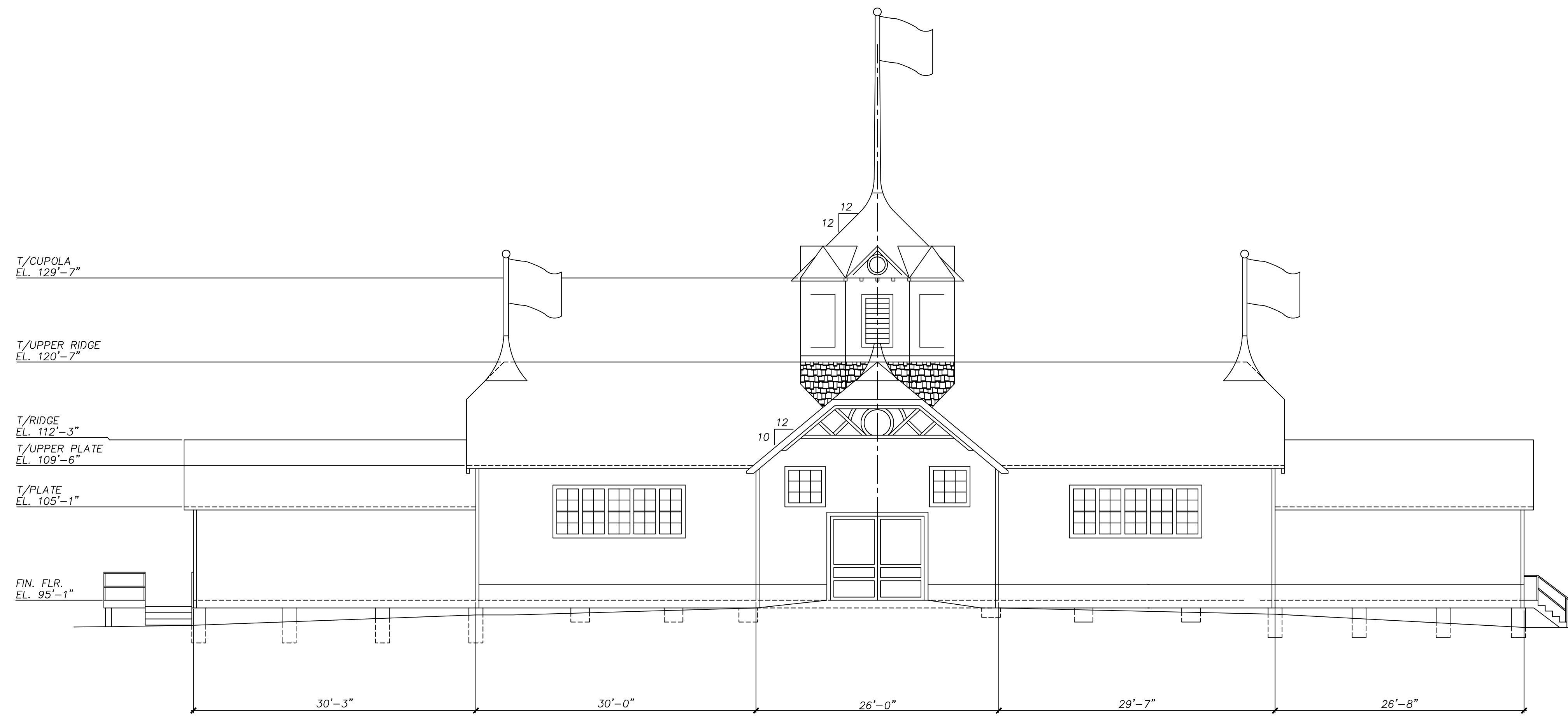
SOUTH ELEVATION
